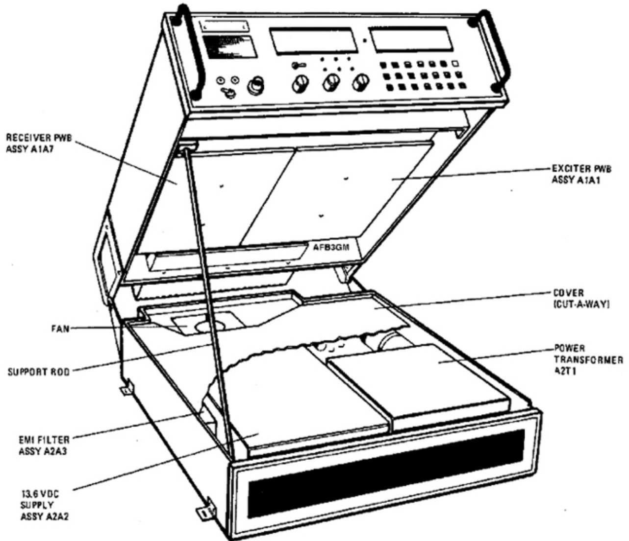
C. TRANSCEIVER ASSEMBLY UNLATCHED AND RAISED
