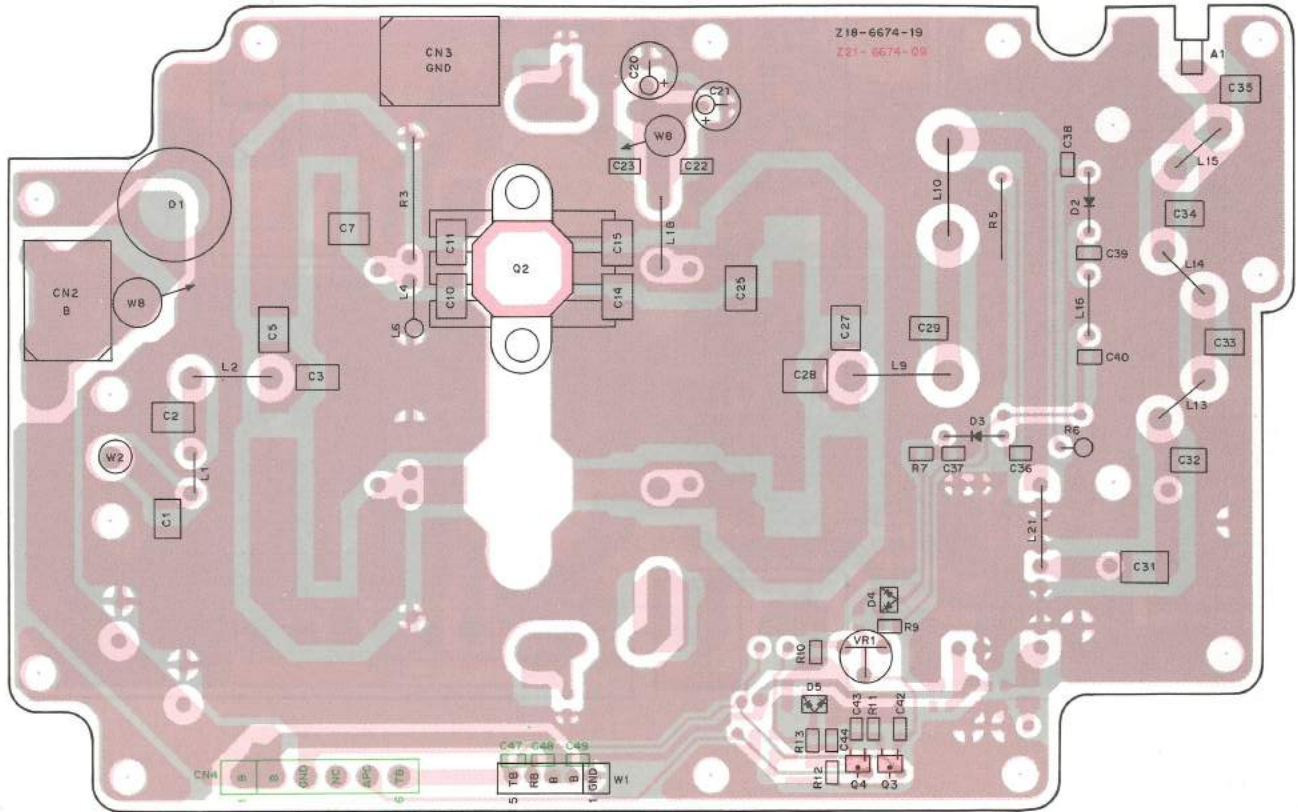
FINAL UNIT (X45-3320-XX) Component side view -11 : K,M,AM,NM -12 : K2,M2,AM2,NM2
