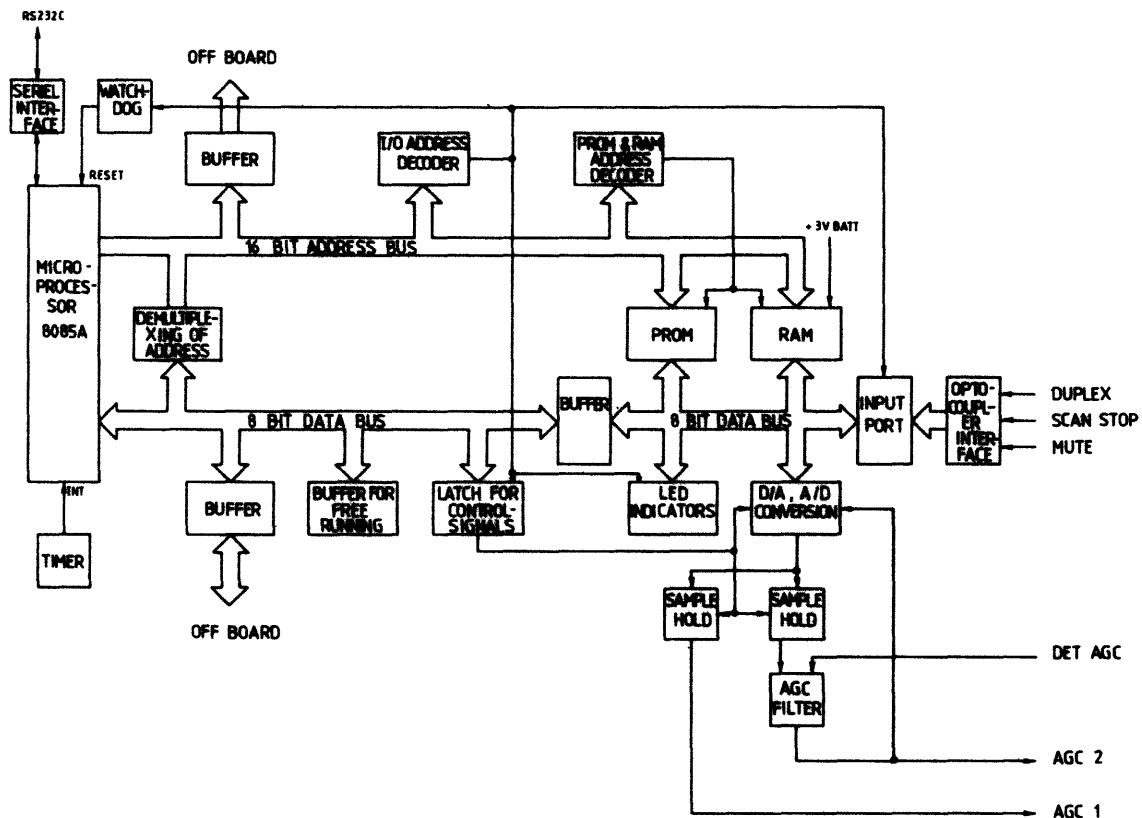
Figure 8.8 Microcomputer Assembly
