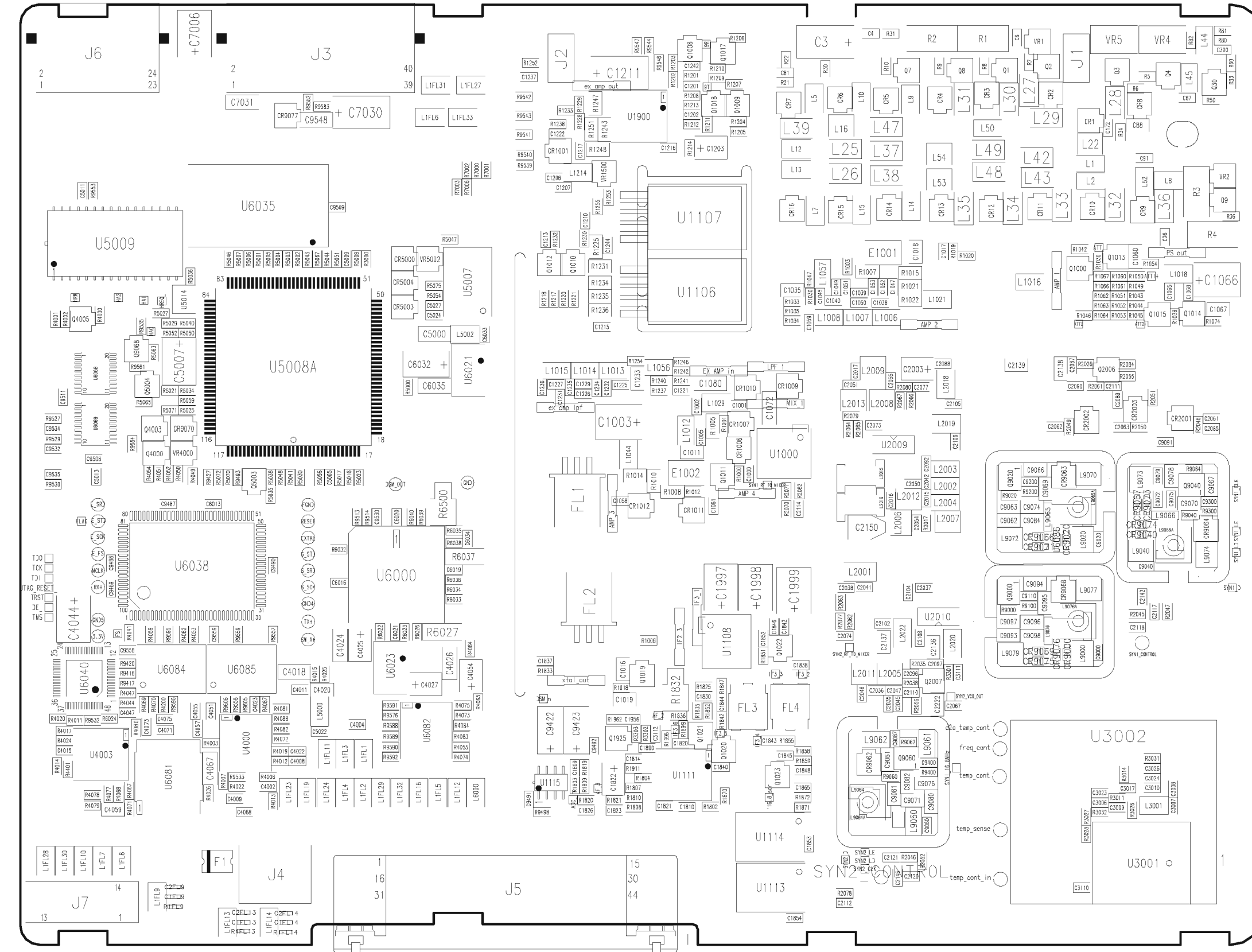
TOP VIEW
