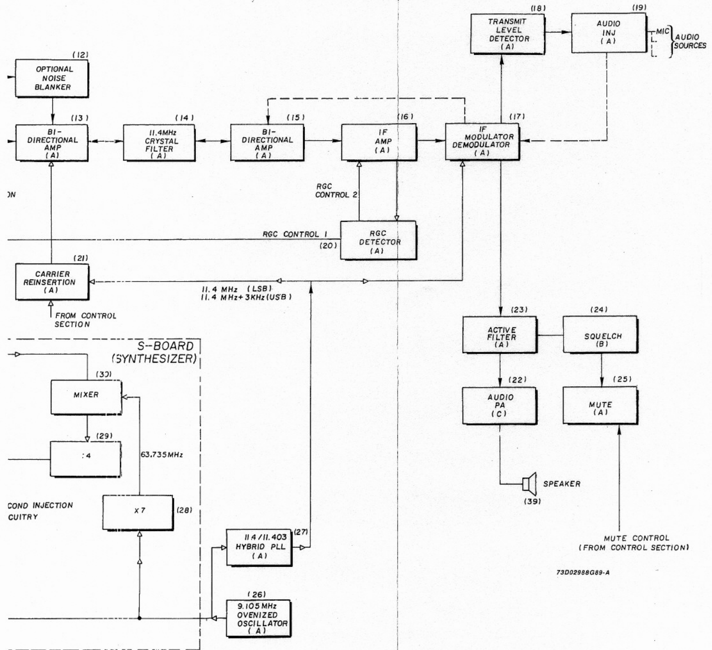
Block Diagram
