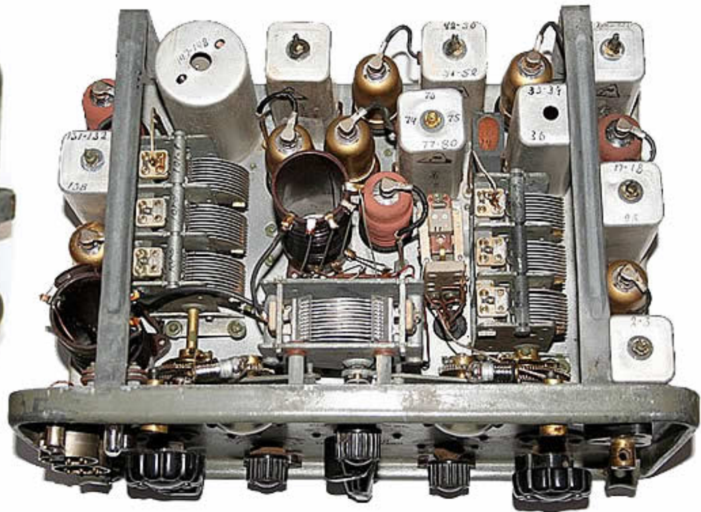
Radio unit RBM-1
