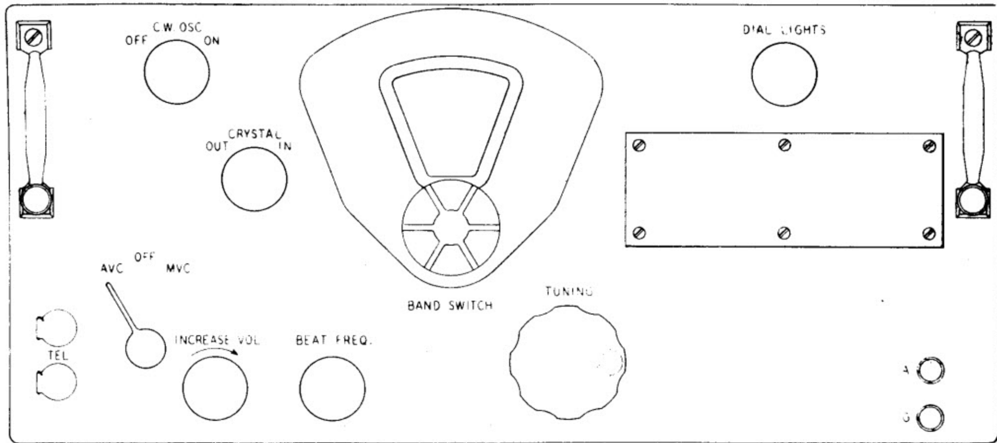
Figure 3 — Radio Receiver BC-348-J, View of Front Panel
