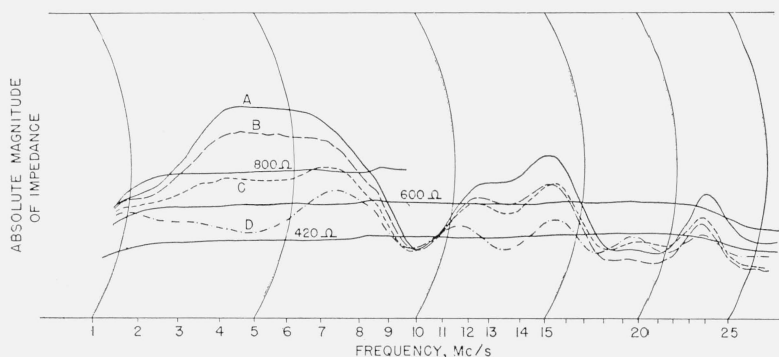
FIGURE 8. Impedance of multiple-wire delta antennas.
