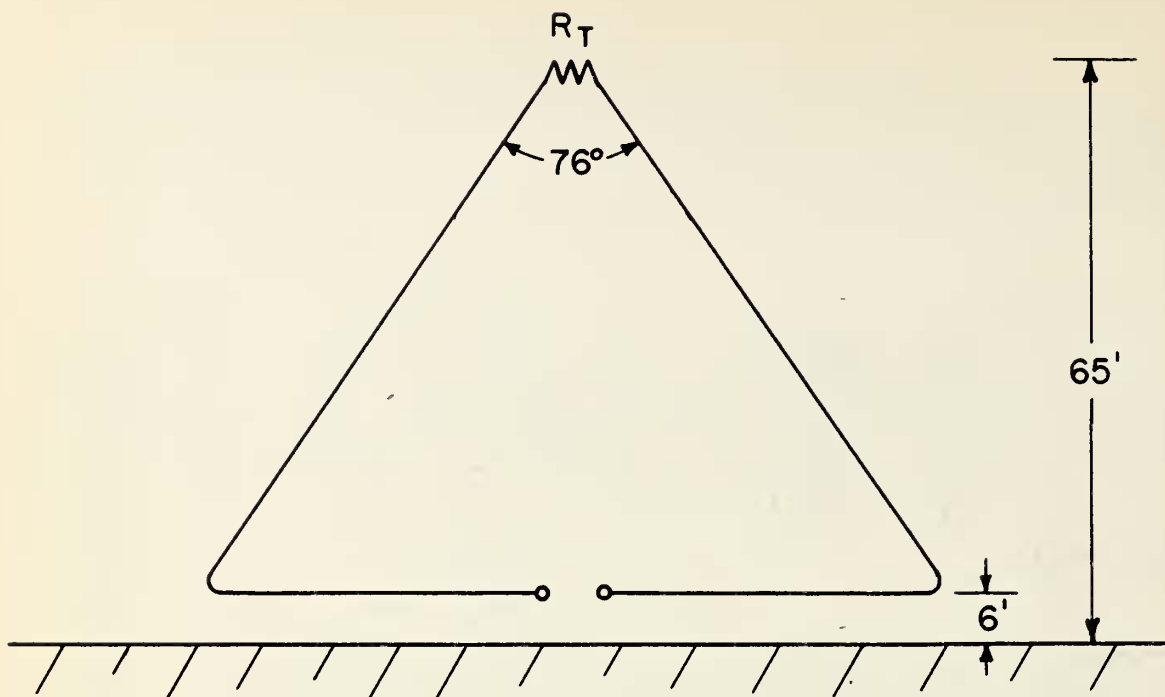
SIDE VIEW
