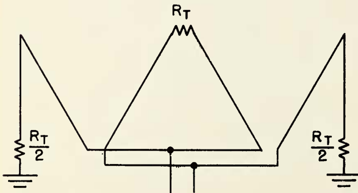
Fig. 8A CONSTRUCTION OF W ANTENNA AND ASSOCIATED TRANSMISSION LINE SYSTEM.
