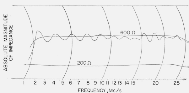
FIGURE 14. Impedance of exponential transmission line.
