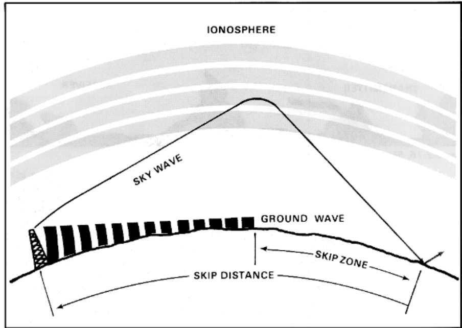
Figure 2- Skip Zones.
