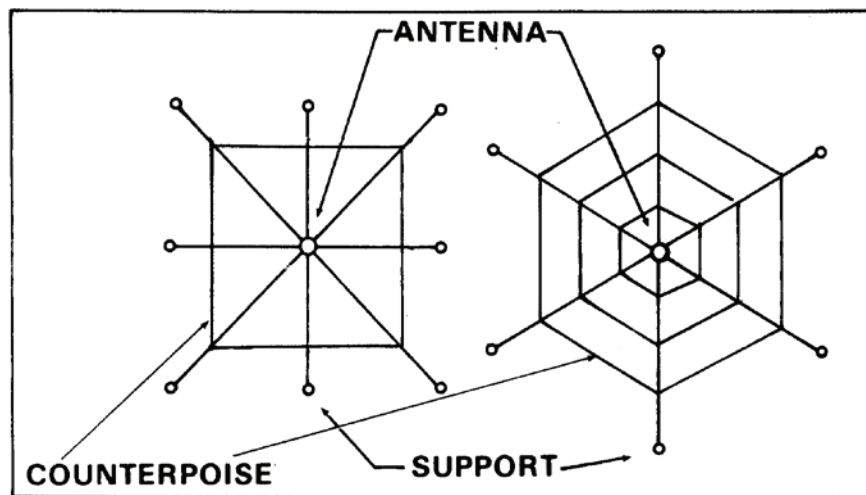
Figure 3-8. Wire counterpoise.
