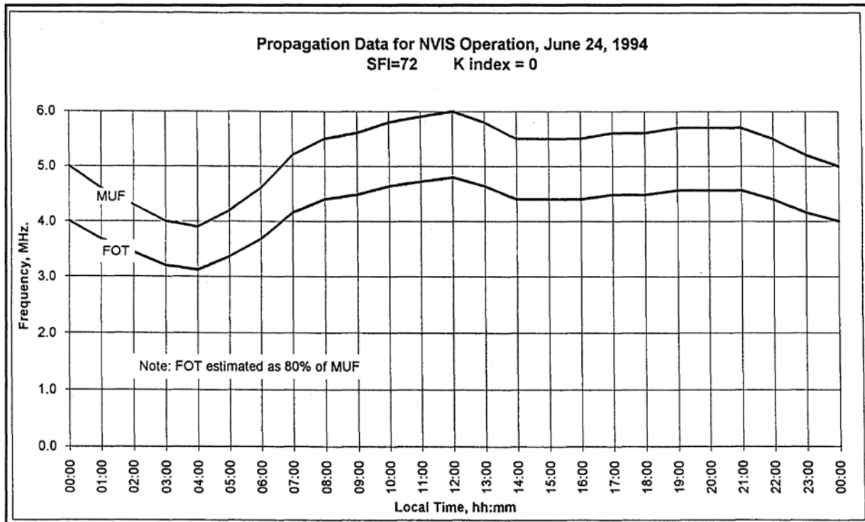
Figure 1. Propagation Conditions
