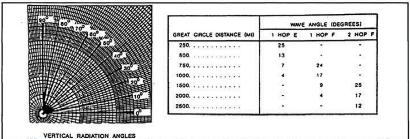
Figure 2. Typical Required Vertical Radiation (Takeoff) Angles for Various Distances In the Northern Temperate Zone
