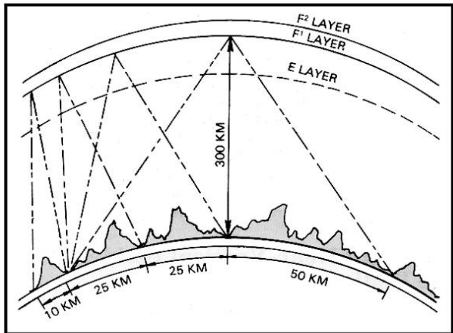
Figure 3 - NVIS Propagation Concept.
