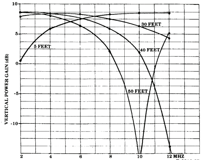
CUT 1/2 λ DIPOLE AT VARIOUS HEIGHTS OVER PERFECT GROUND
