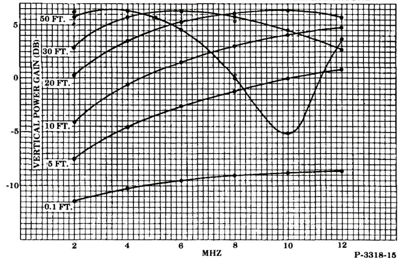
Figure 2. CUT 1/2 λ DIPOLE AT VARIOUS HEIGHTS OVER AVERAGE GROUND
