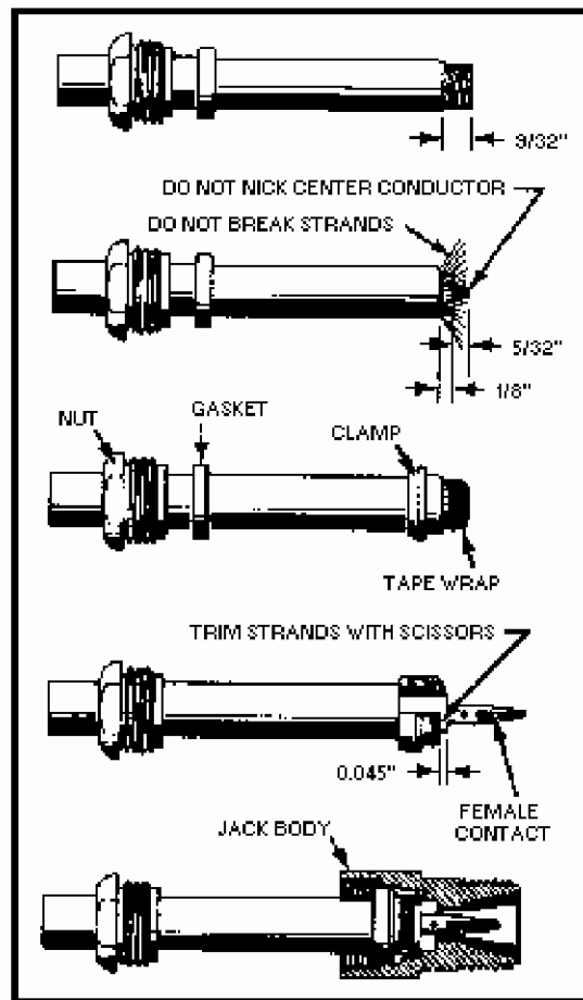
Figure 1-30.—Attaching N connectors to coaxial cable.
