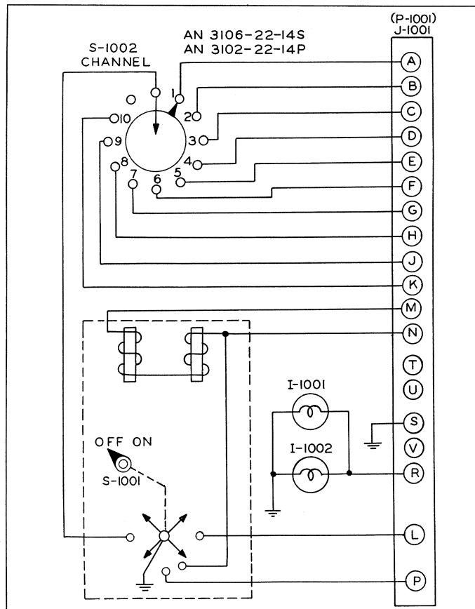
Figure 8-14. Radio Set Control C-733/ARR-15A, Schematic Wiring Diagram
