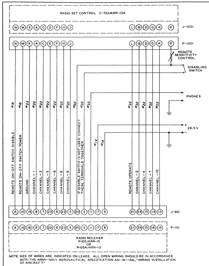
Figure 8-11. External Connections to R-105/ARR-15 Receiver
