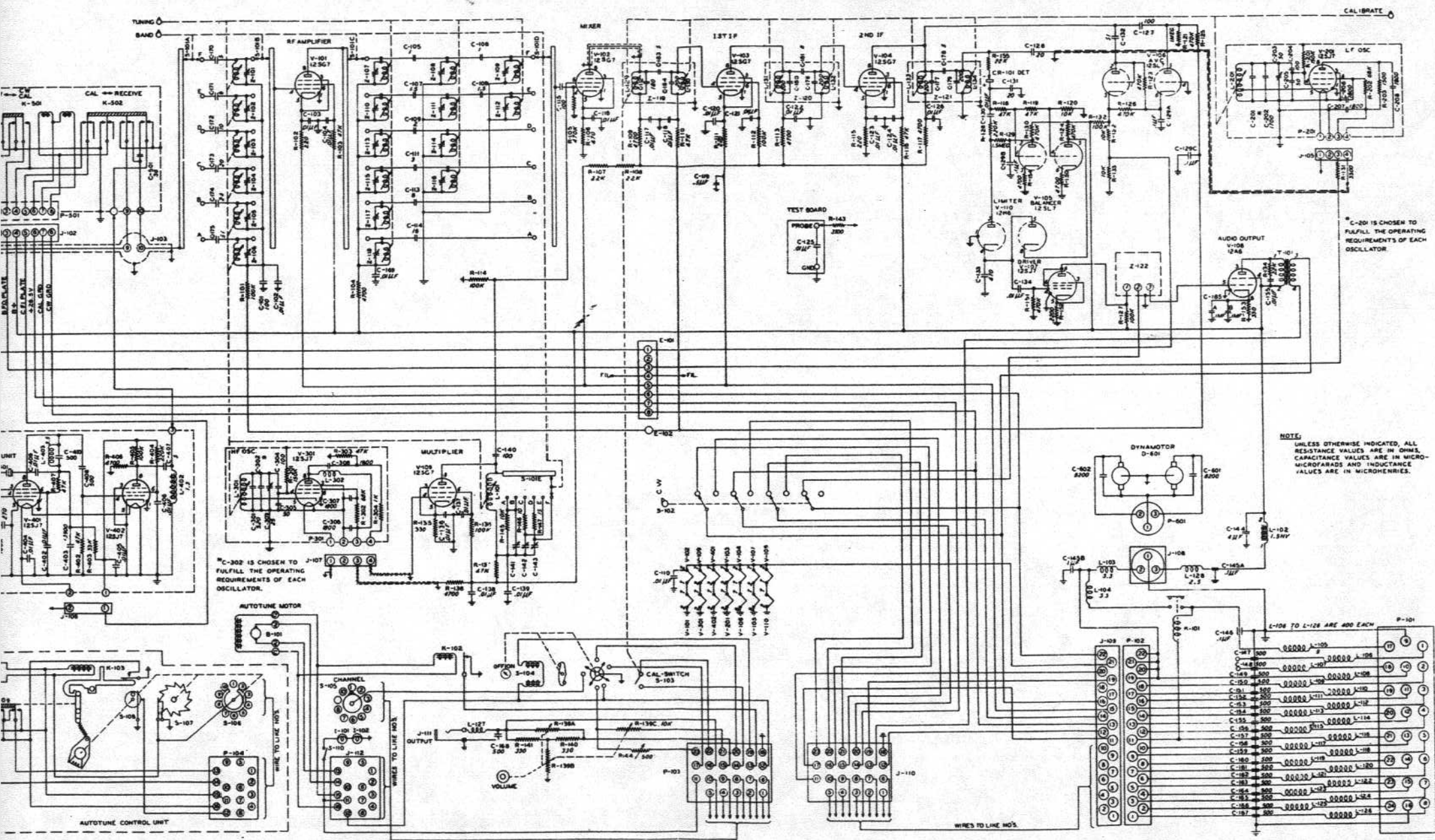
Figure 8-9. Receiver Complete Schematic Wiring Diagram
