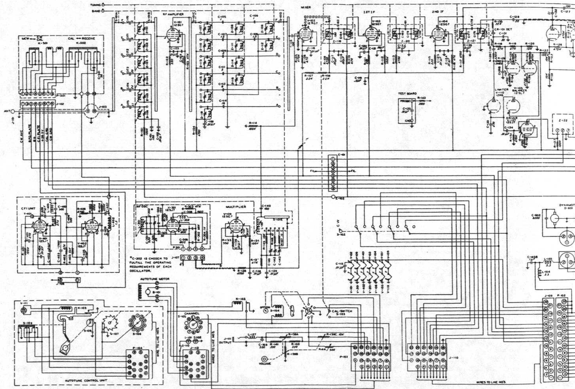
Figure 8-9. Receiver Complete
