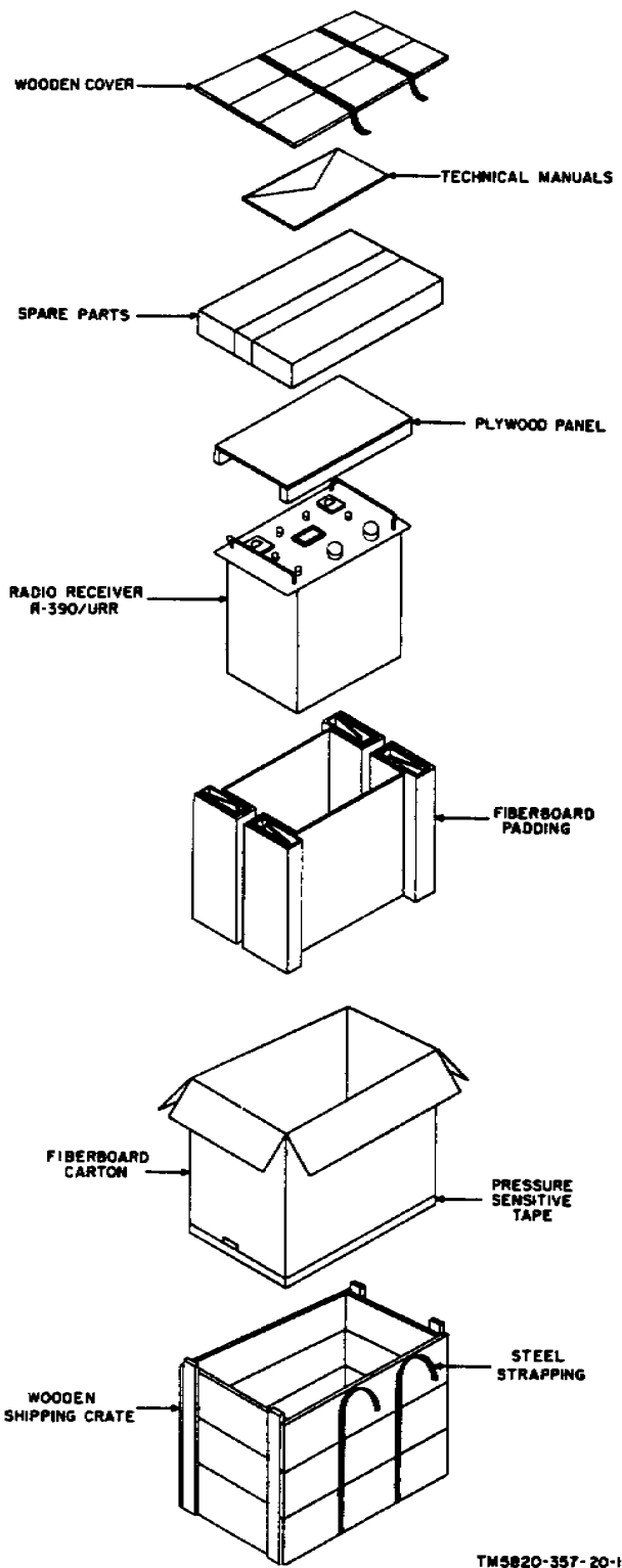
Figure 1. Unpacking
