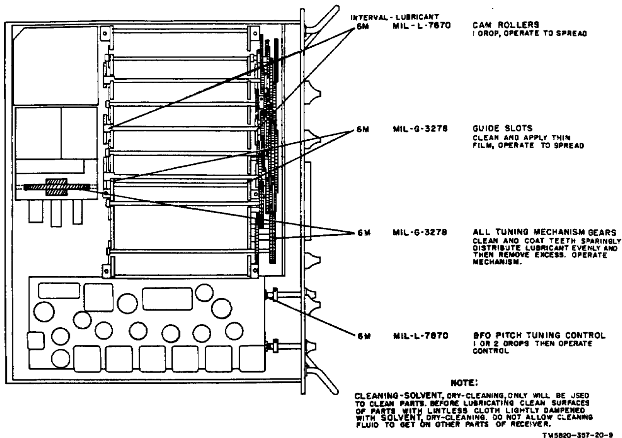
Figure 7. Lubrication.
