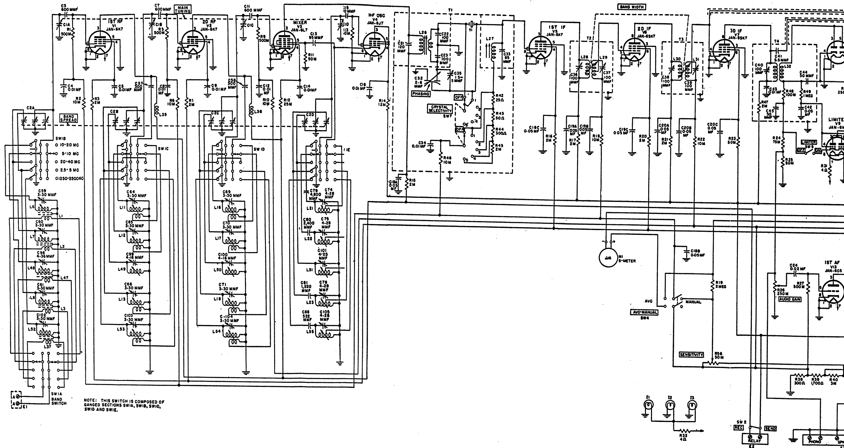
Figure 57. Radio Receiver BC-794-A, -B, schematic diagram.
