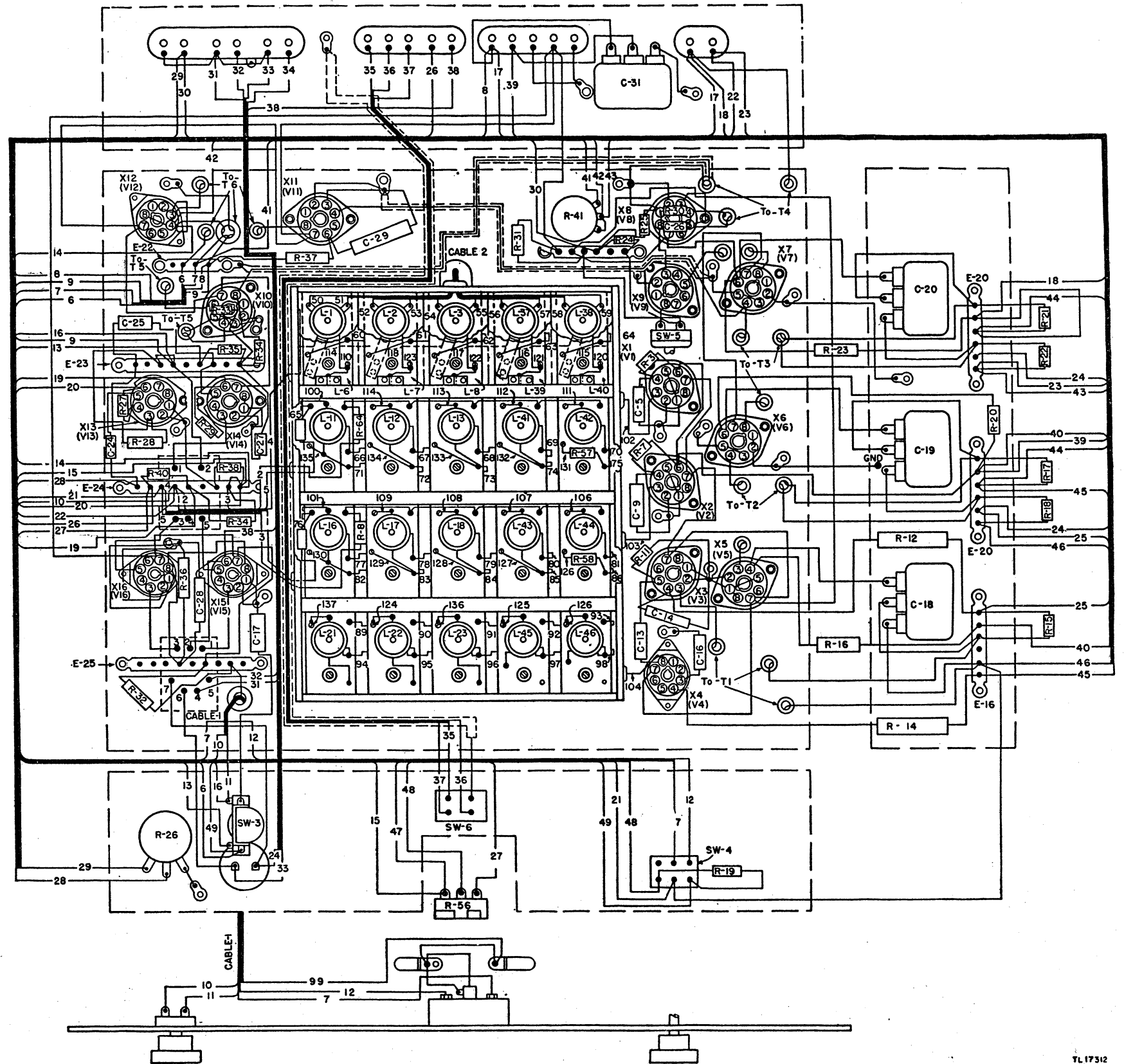
Figure 60. Receiver chassis, wiring diagram.
