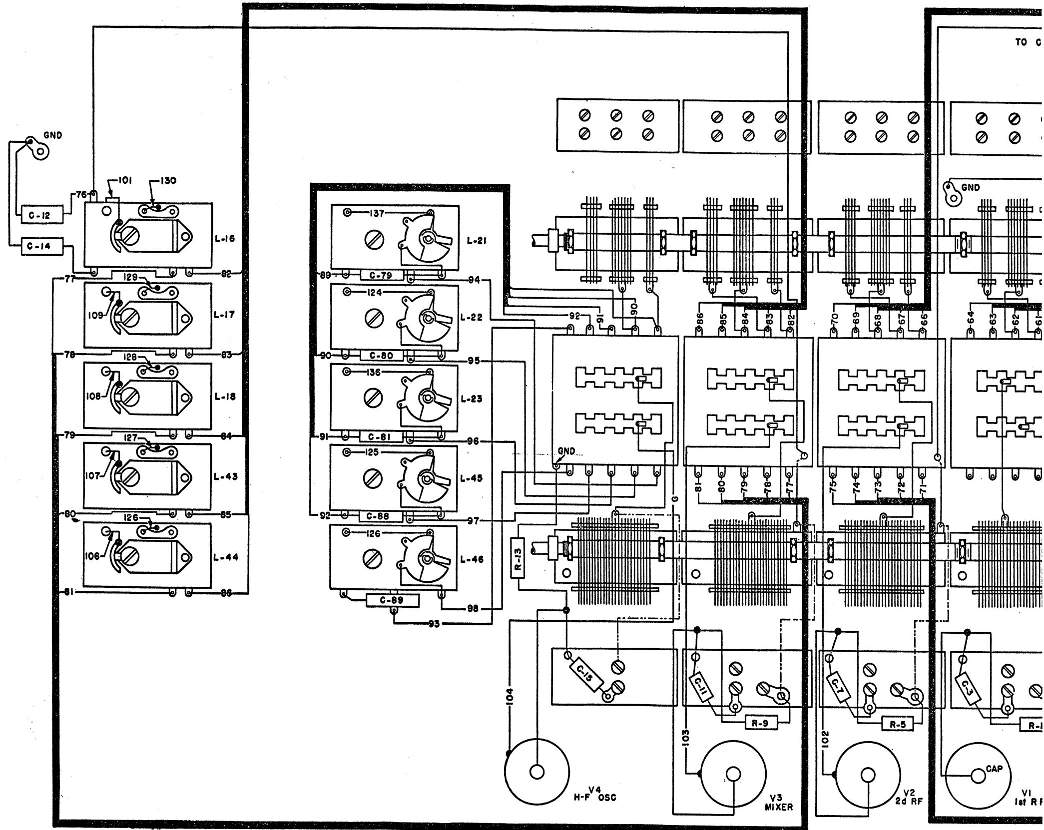
Figure 61. Receiver tuning unit, wiring diagram.
