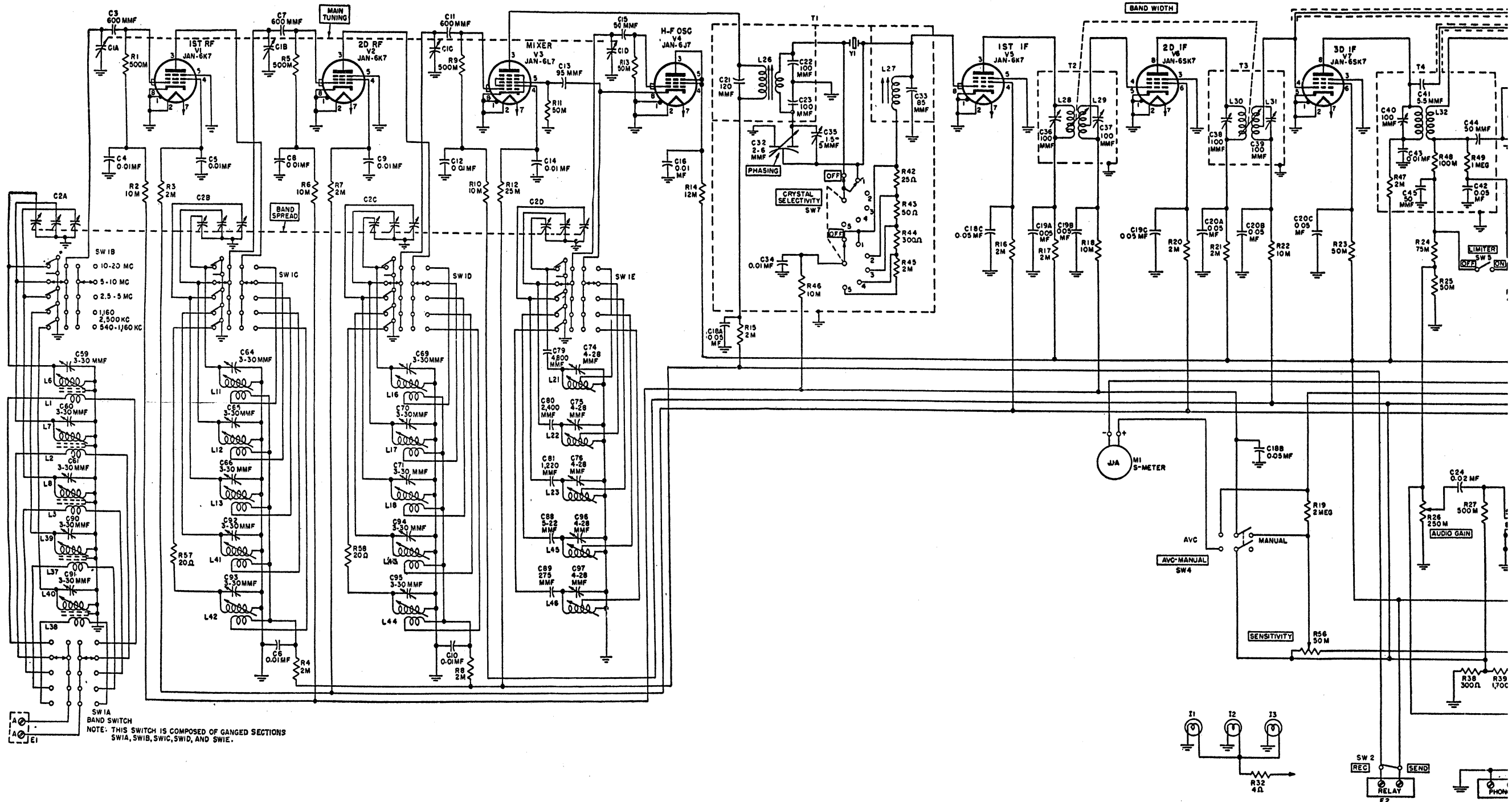
Figure 58. Radio Receiver BC-100A-B, -C, schematic diagram.
