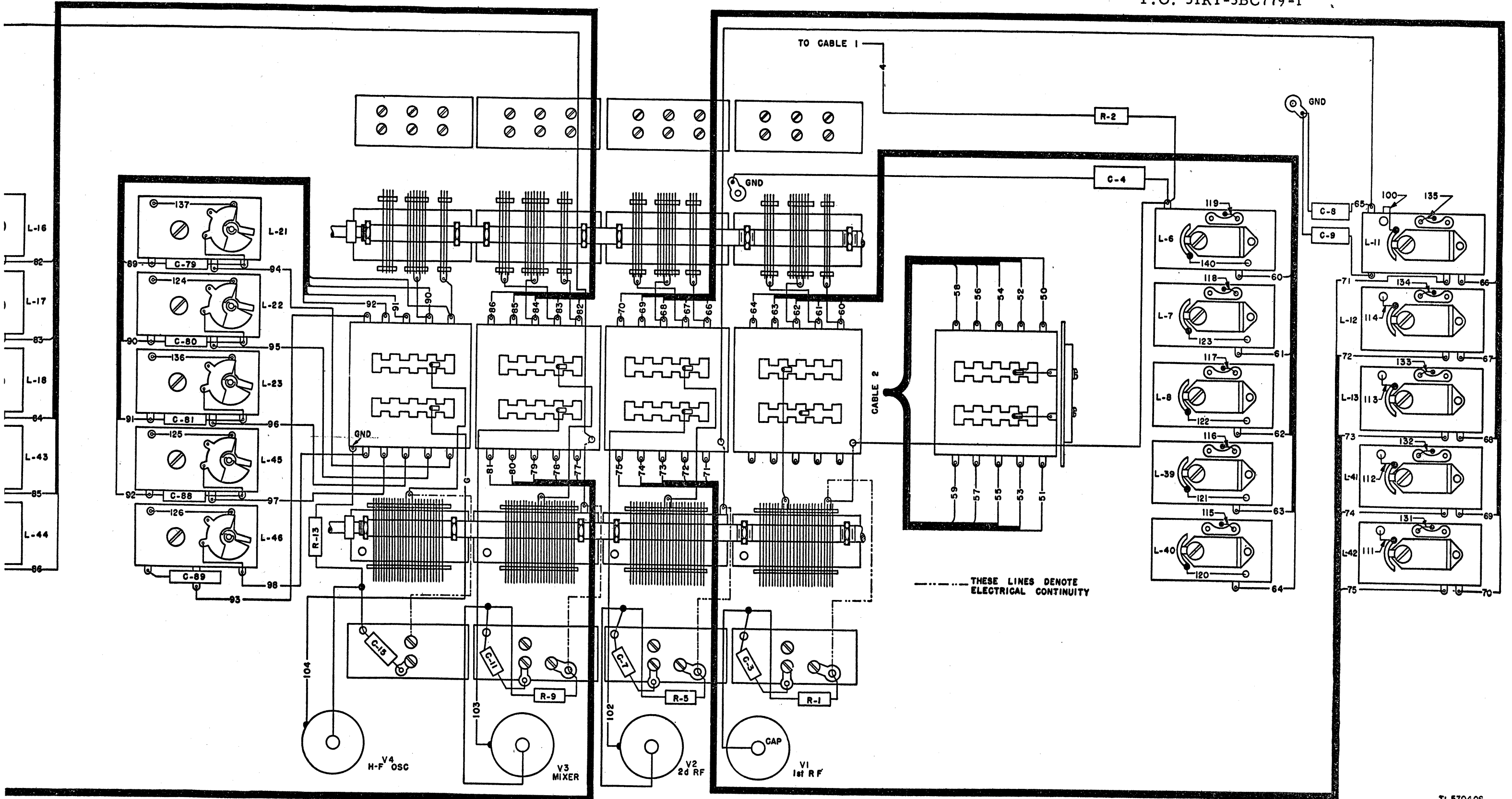
Figure 61. Receiver tuning unit, wiring diagram.
