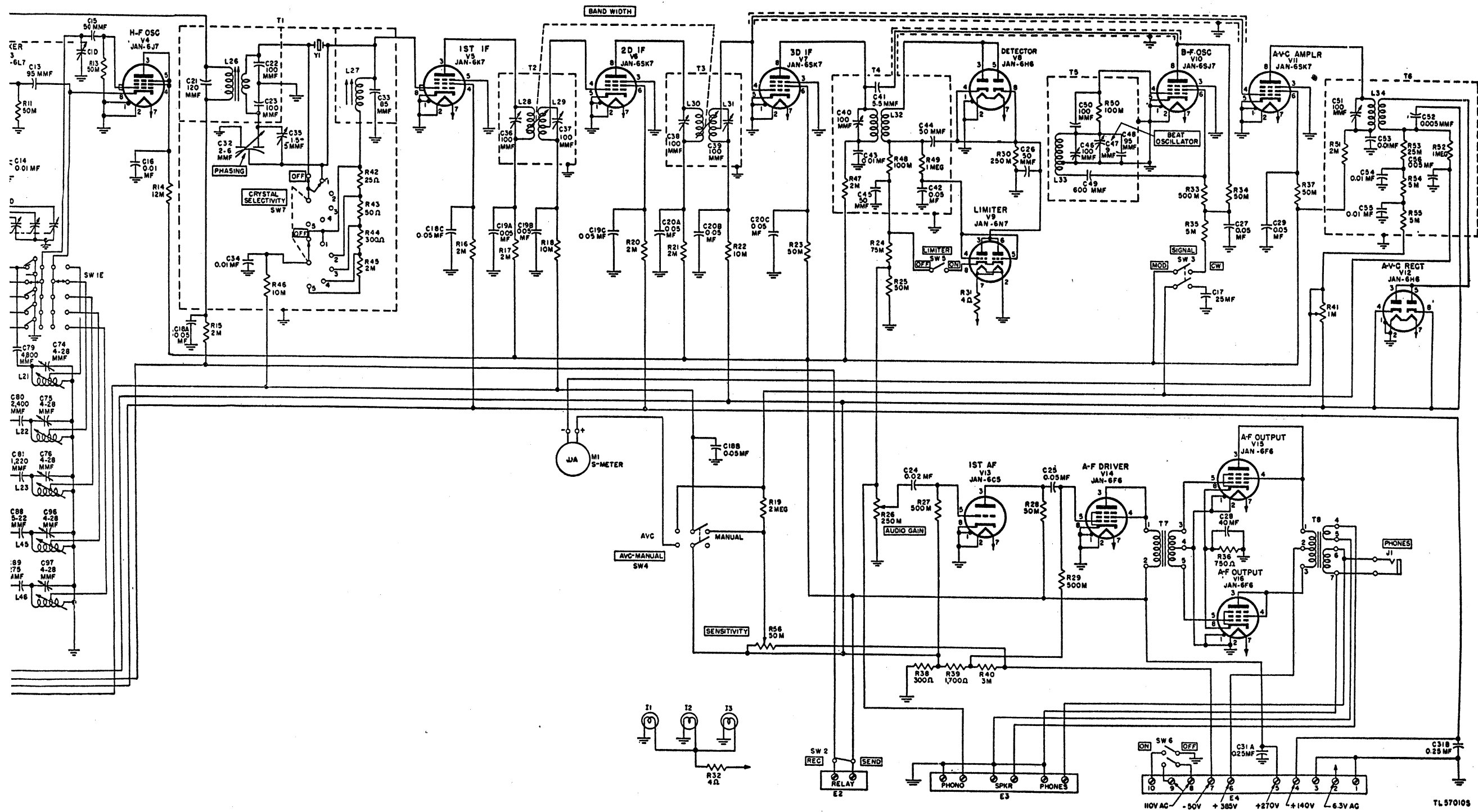
Figure 58. Radio Receiver BC-1004-B, -C, schematic diagram.
