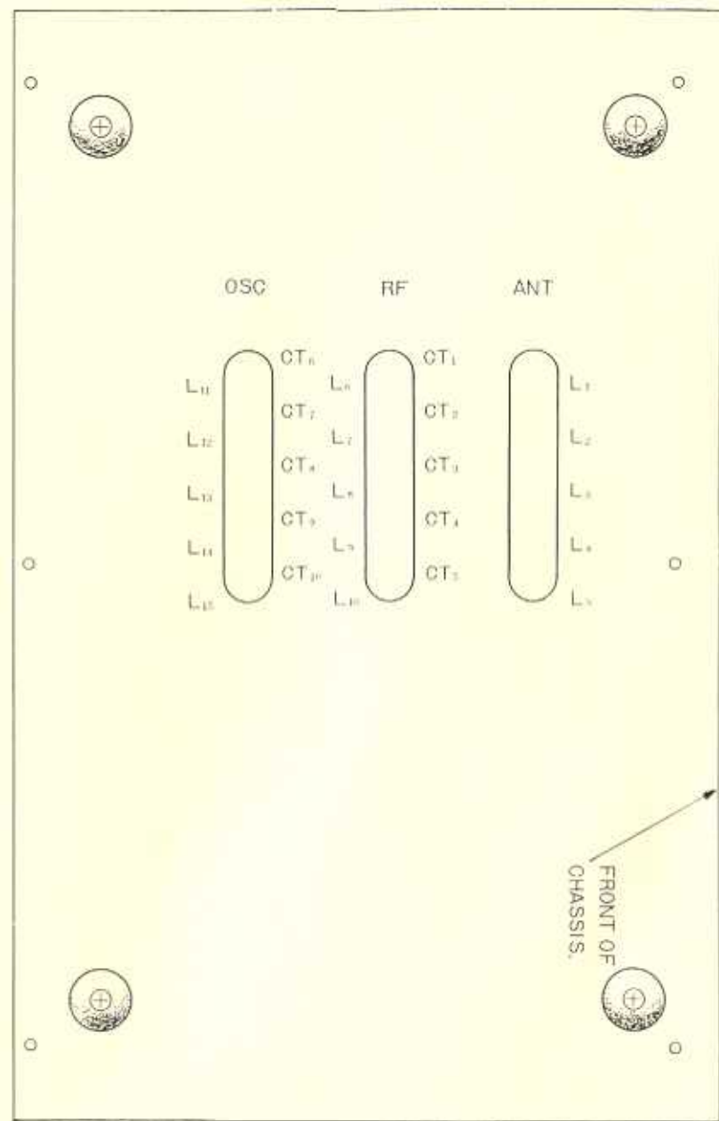
ALIGNMENT POINTS (BOTTOM VIEW)
