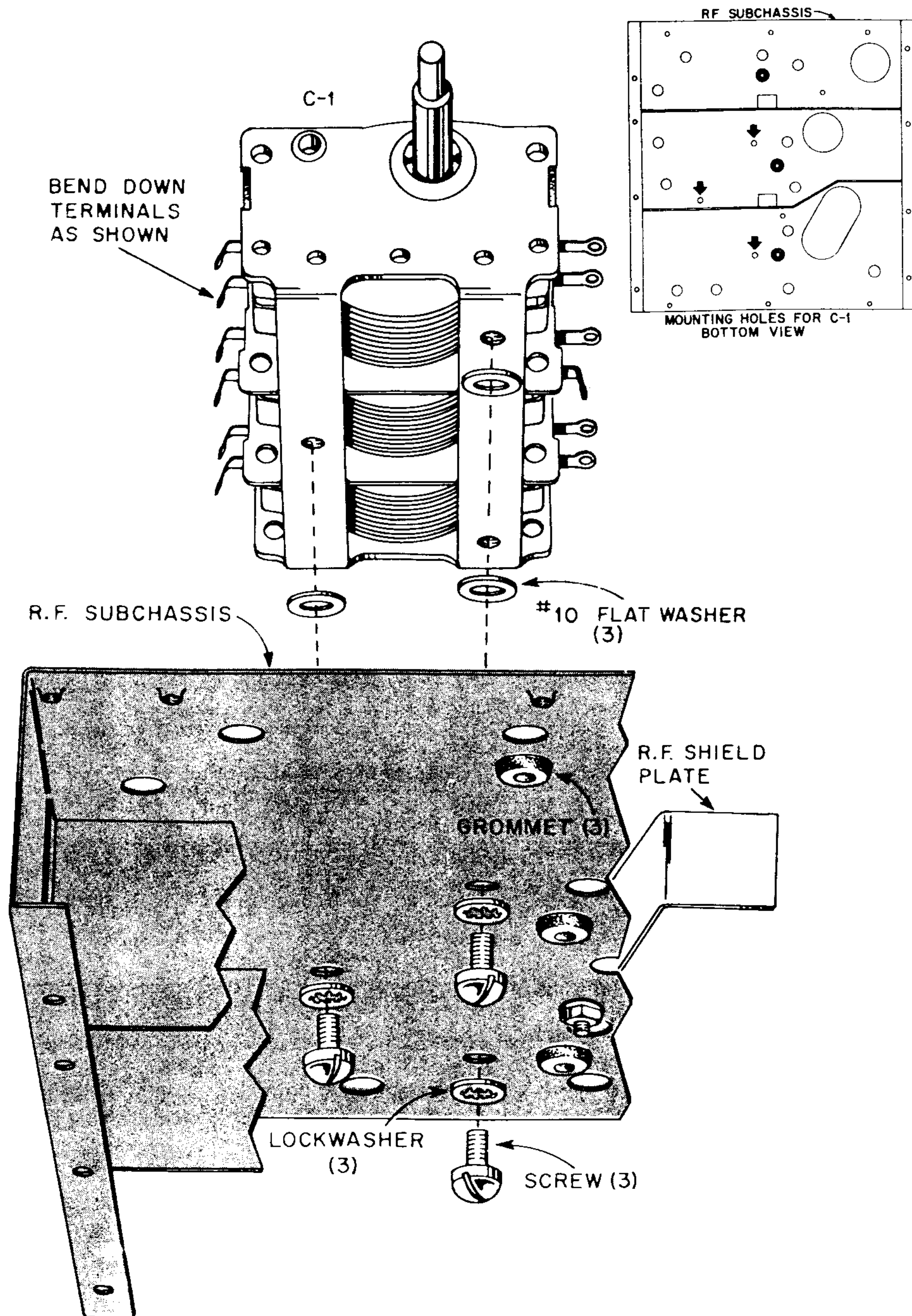
FIGURE 17. MOUNTING C-1 (MAIN TUNING CAPACITOR)
