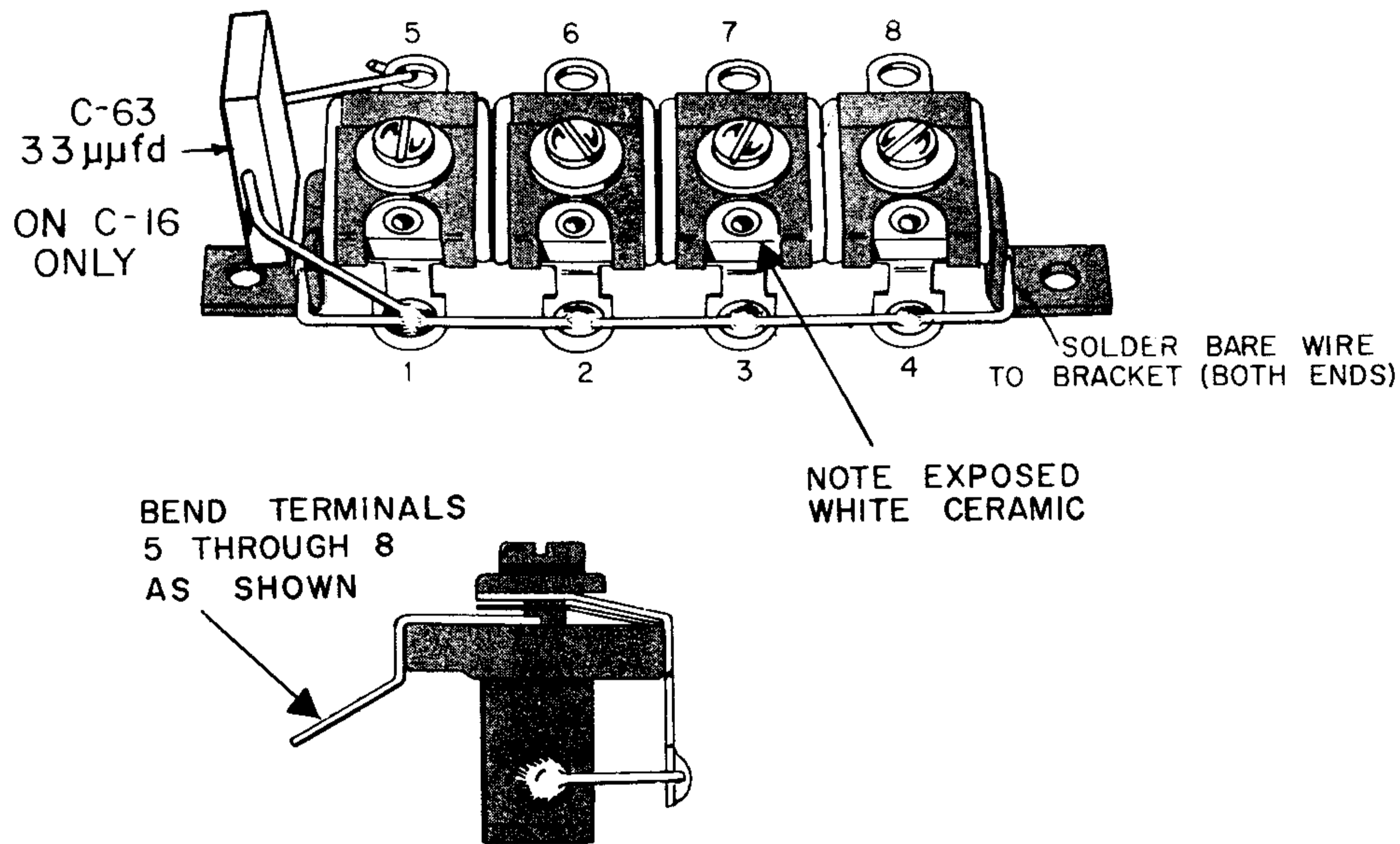
END VIEW FIGURE 14. PREPARING THE TRIMMER STRIPS
