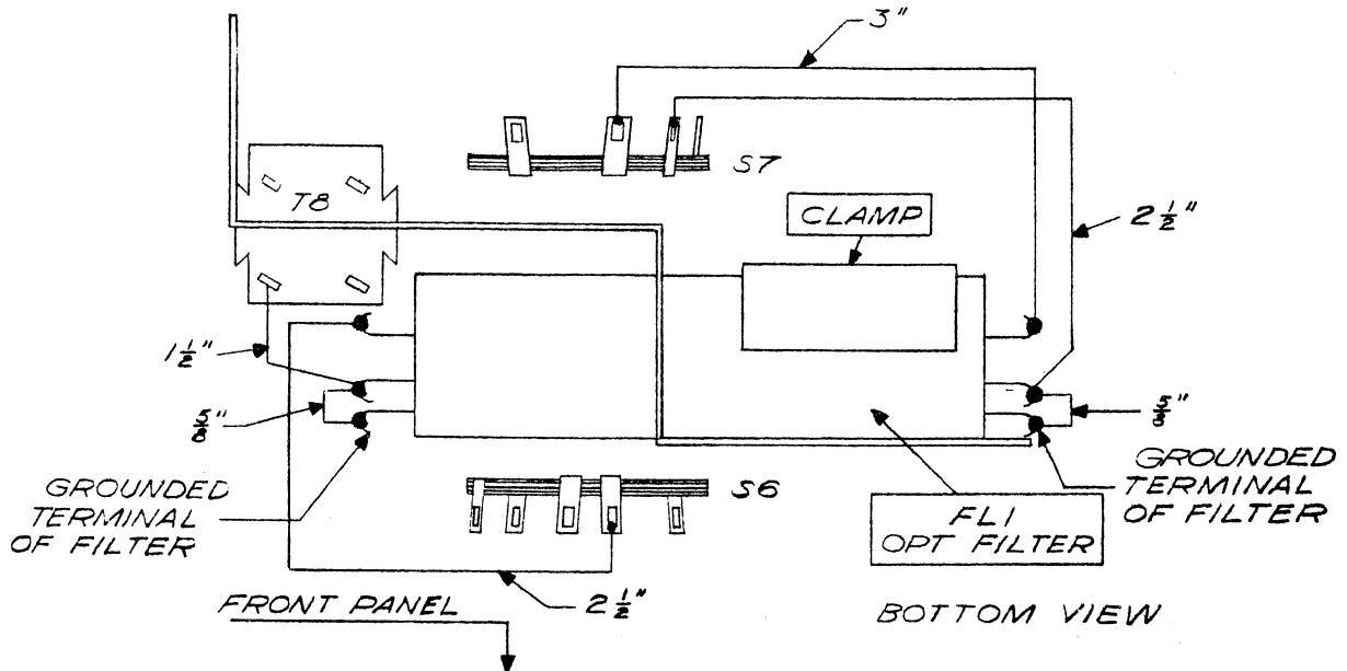
Collins Type F455Q-5 Mechanical Filter, part number 526 9367 00 (Install in either direction)
