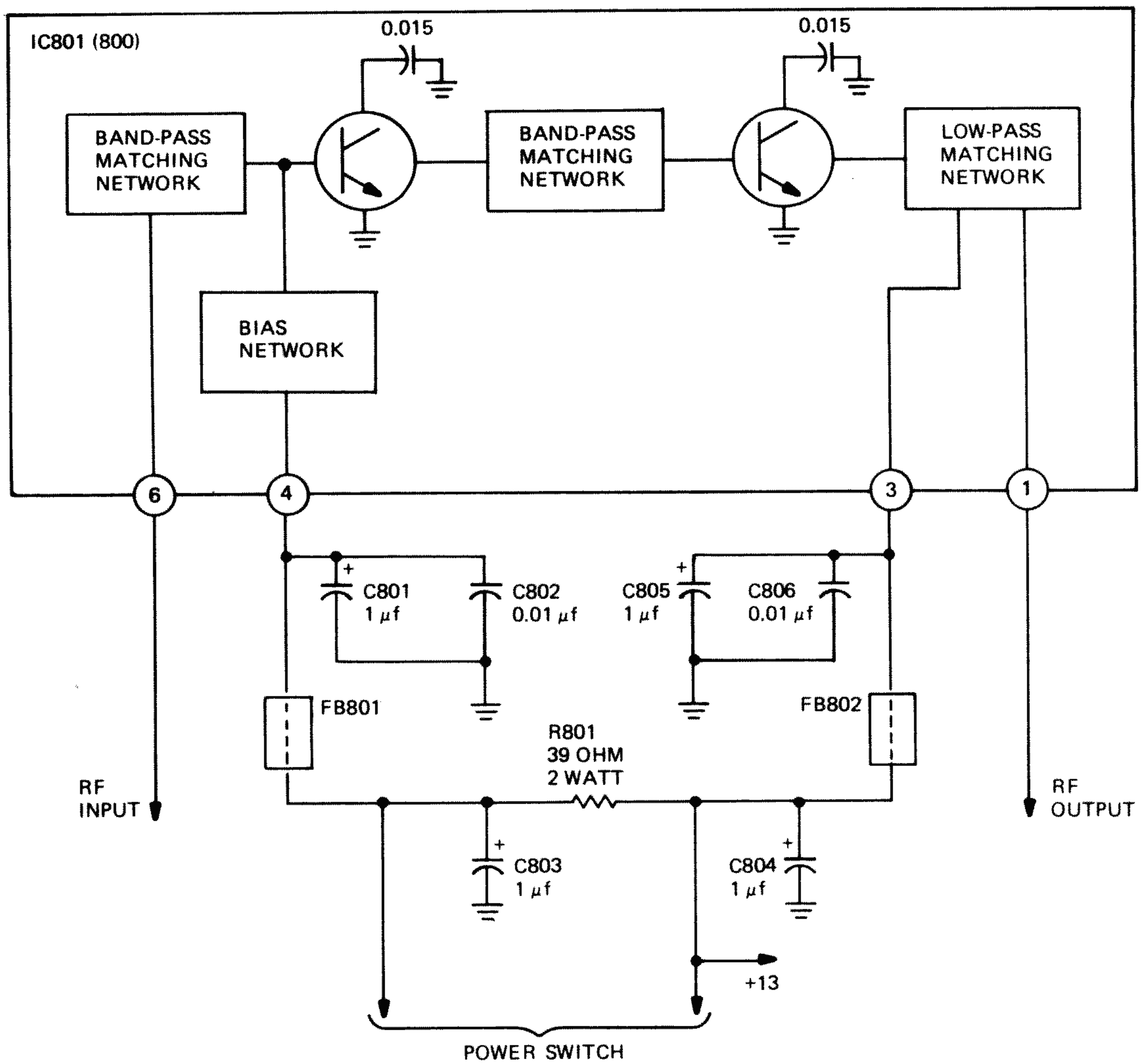
Fig. 29. Power amplifier schematic.
