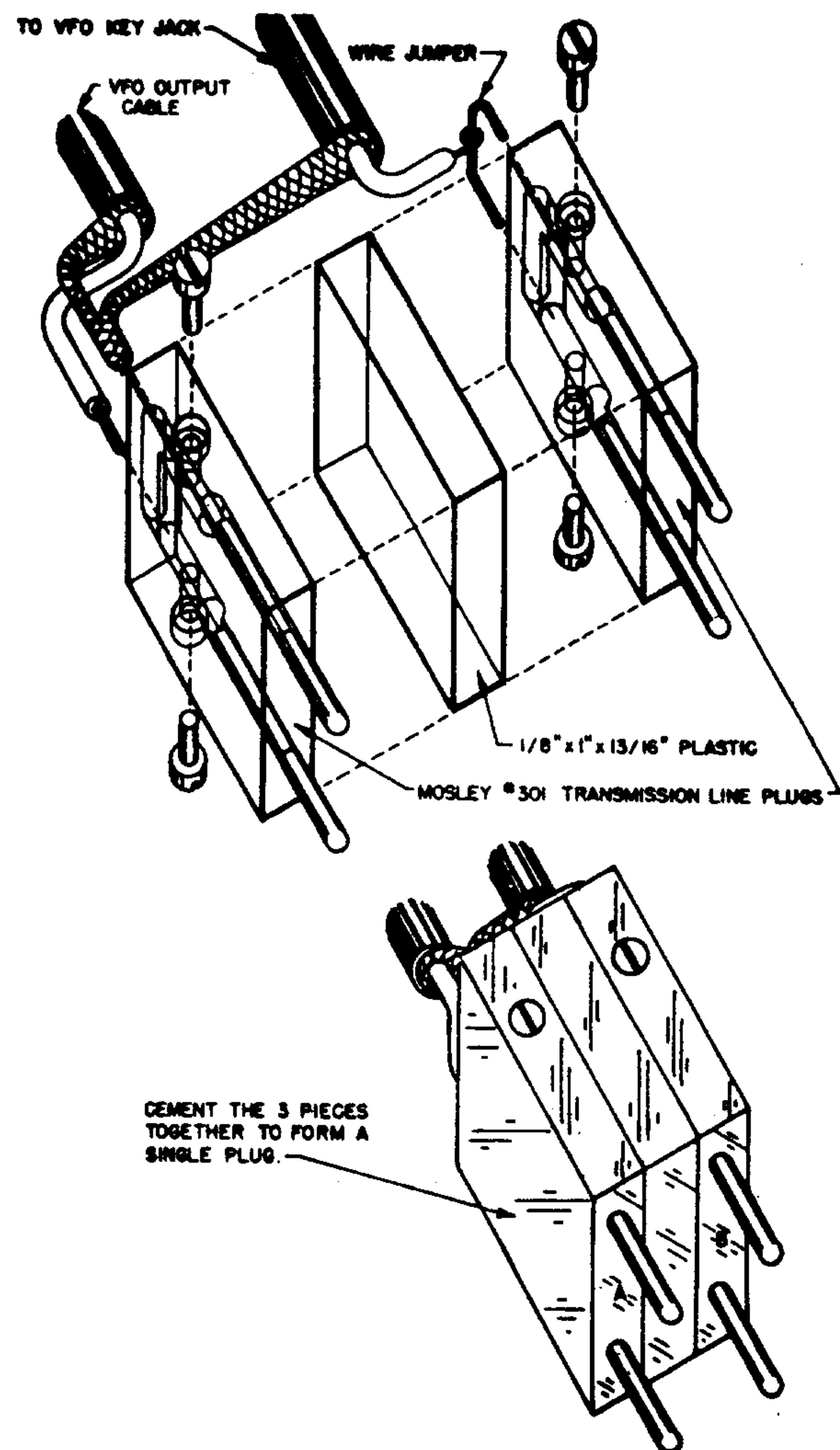
Figure 1 Jumper Plug
