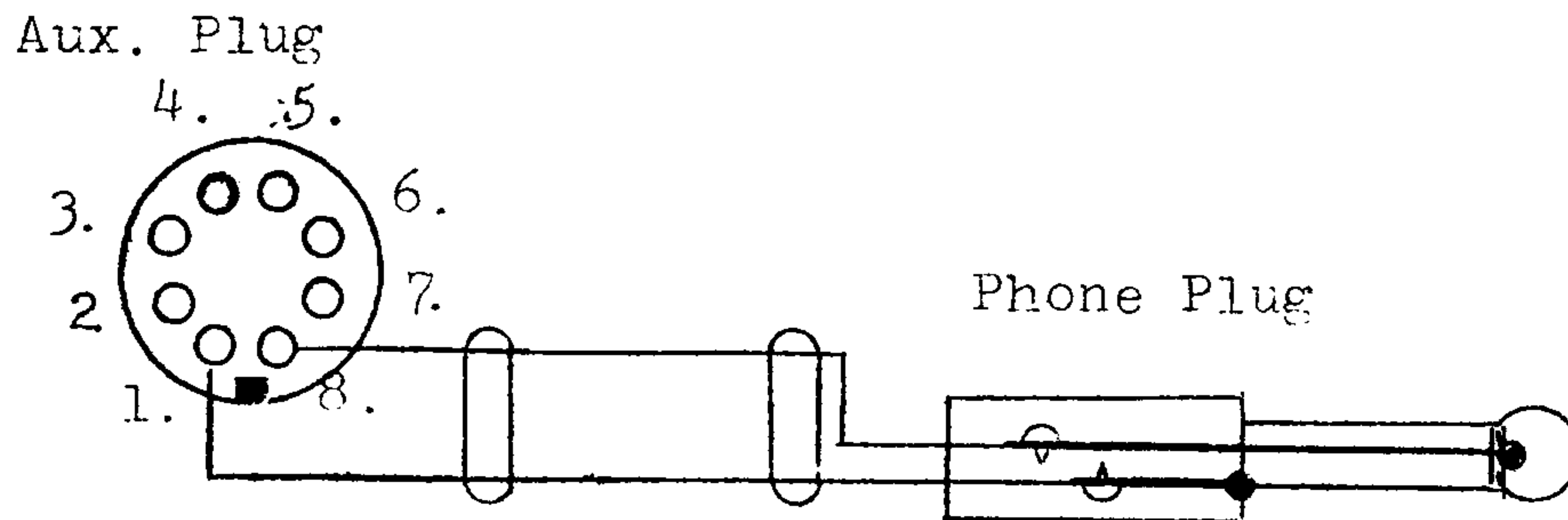
Figure 3 Automatic Phone Operation Cord
