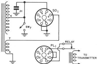
Figure 13. Schematic Remote Control Operation
