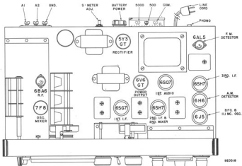
Figure 12. Top view of Chassis
