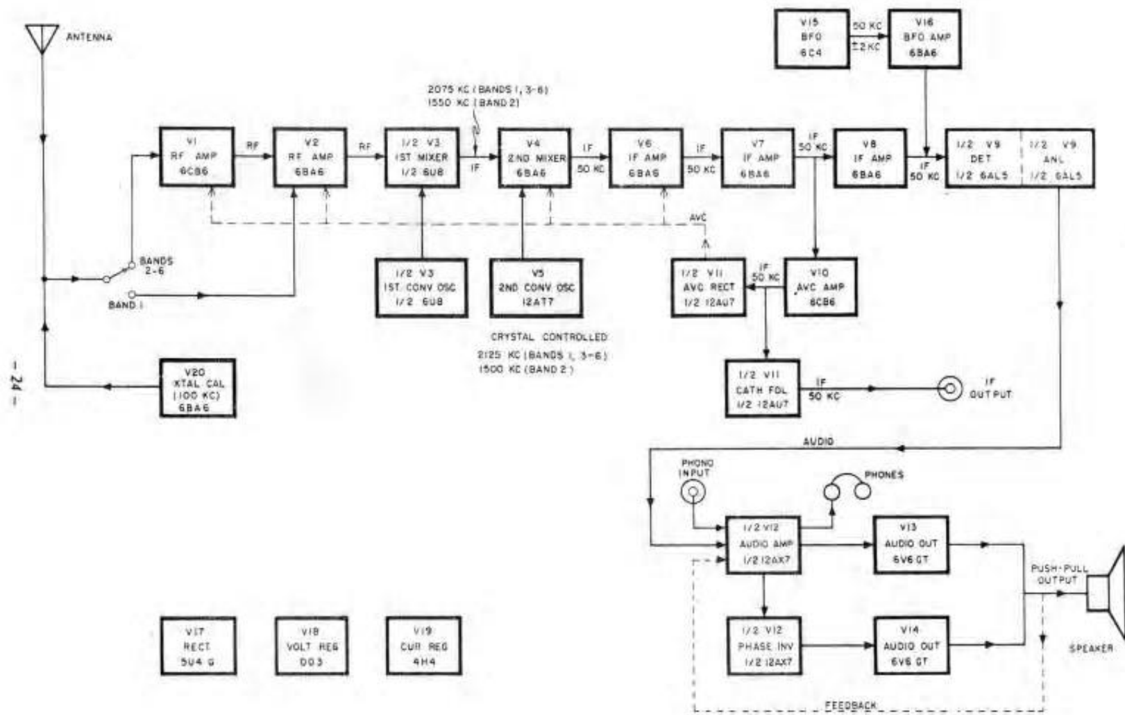
Fig. 14. Block Diagram of Receiver
