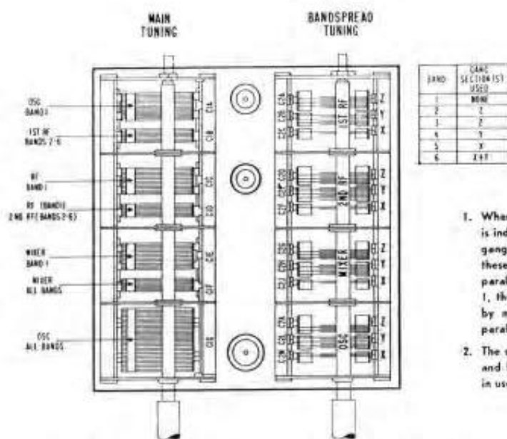
Fig. 15. Location and Function of Tuning Gang Sections
