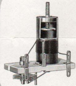
TUNING COIL UNIT
