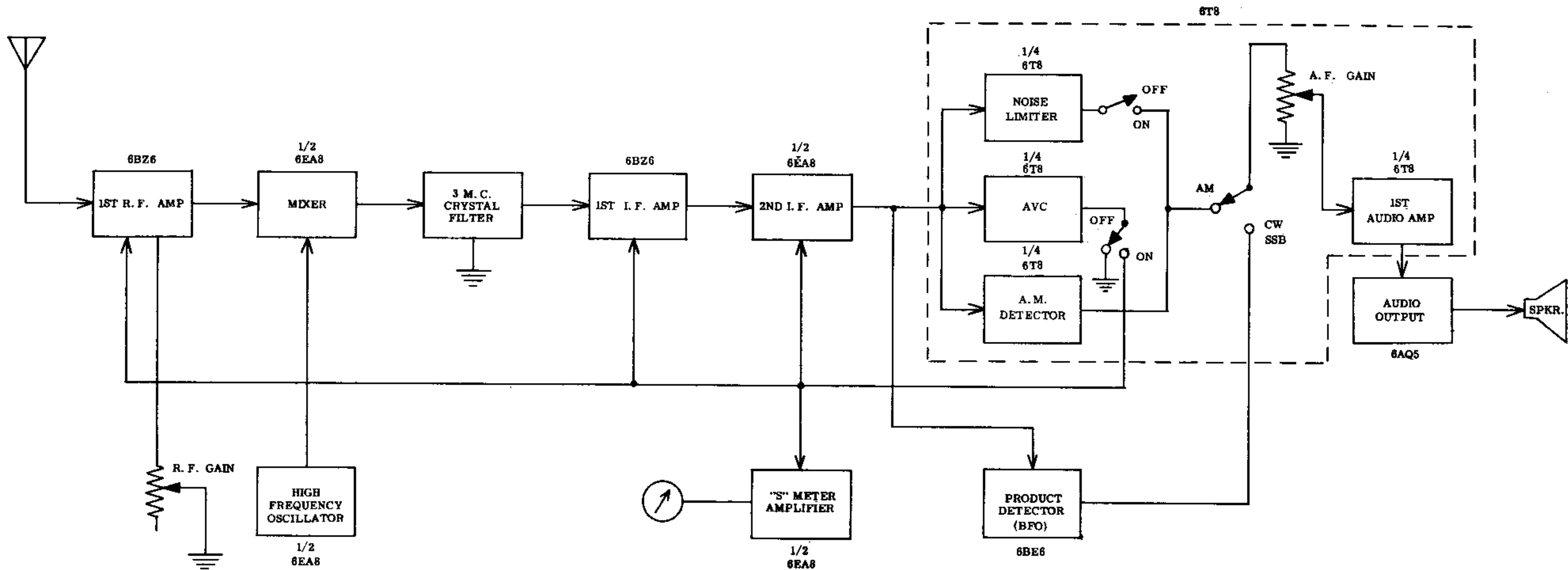
BLOCK DIAGRAM
