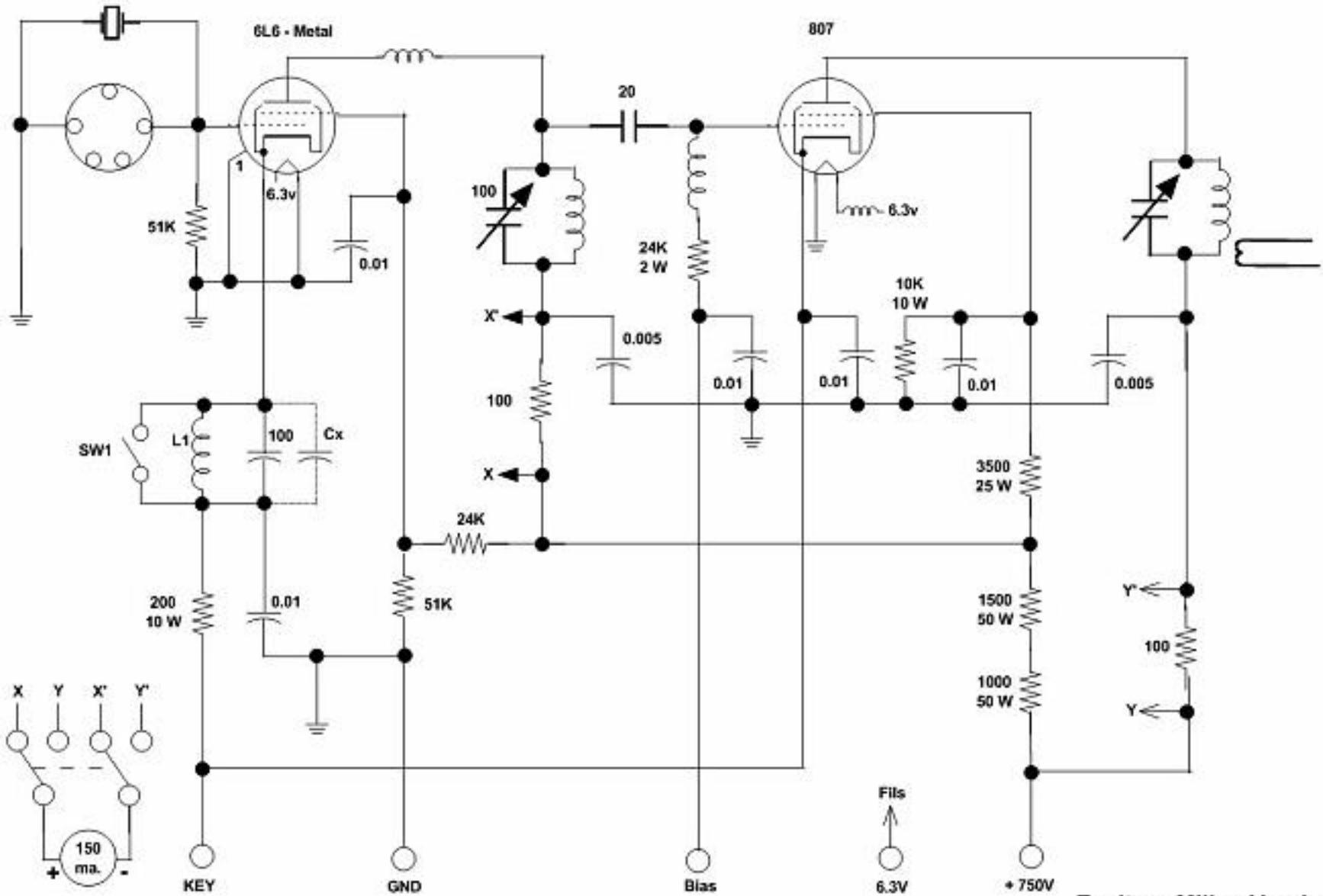
Exciter - Millen Version Serial # 459 10/2/1945
