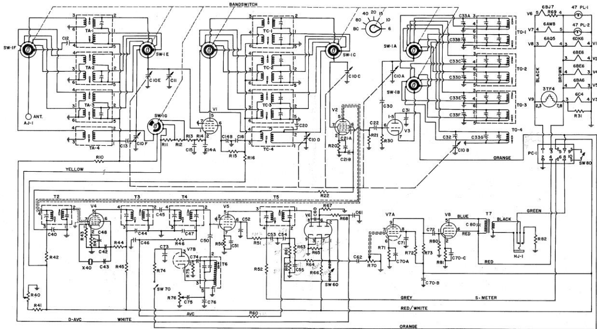
PMR-8 SCHEMATIC
