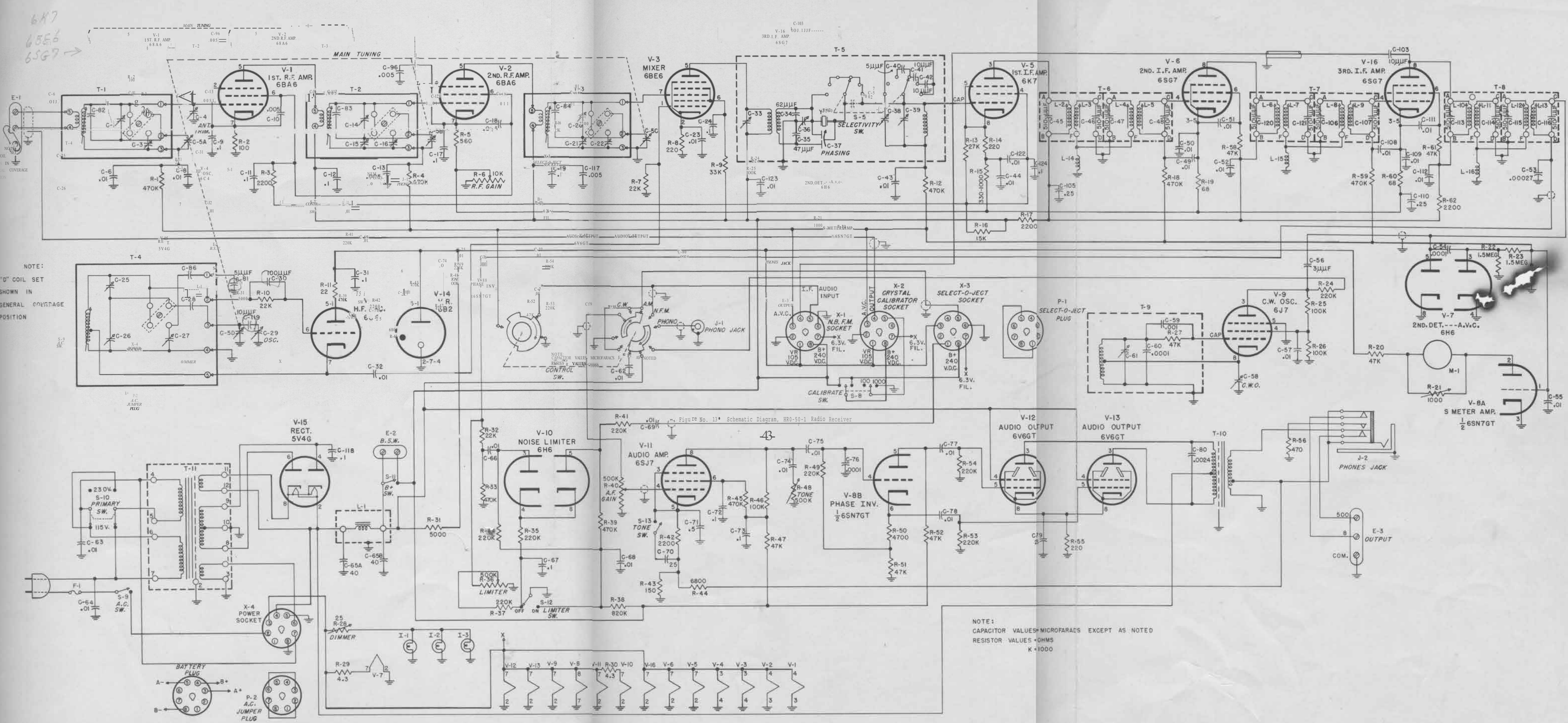
Figure No. 13. Schematic Diagram, HR0-50-1 Radio Receiver
