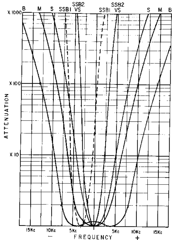
Figure 2. IF Selectivity Curves
