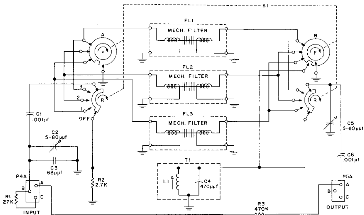
Figure 11. Schematic, MFH Mechanical Filter Housing
