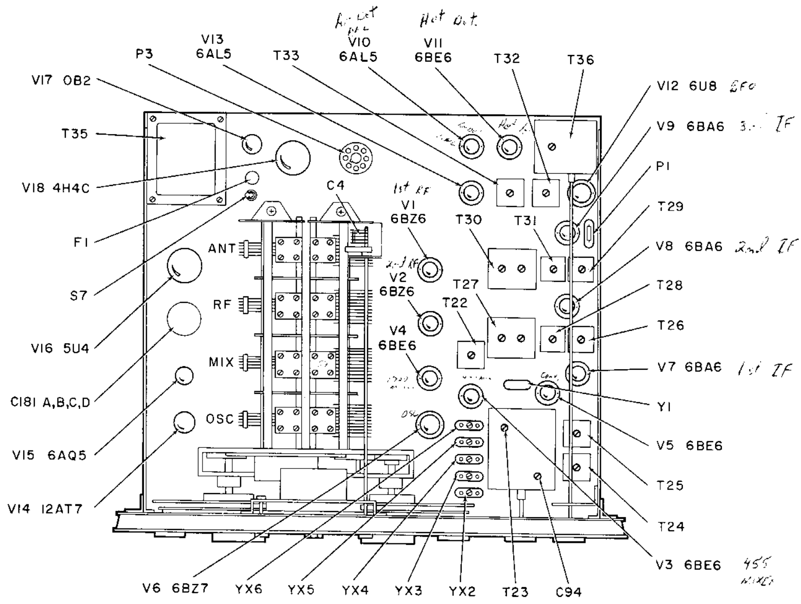
Figure 6. Tube Locations and Alignment Adjustments
