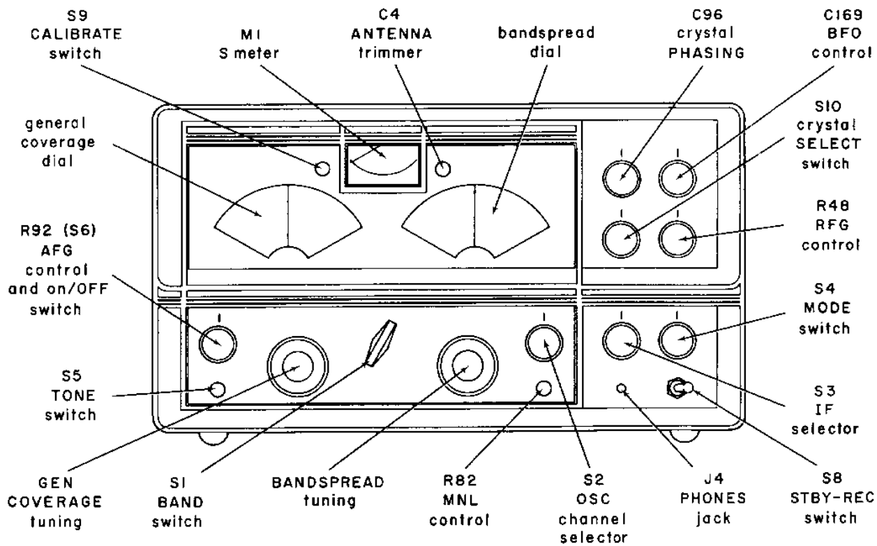
Figure 5. Panel Control Locations
