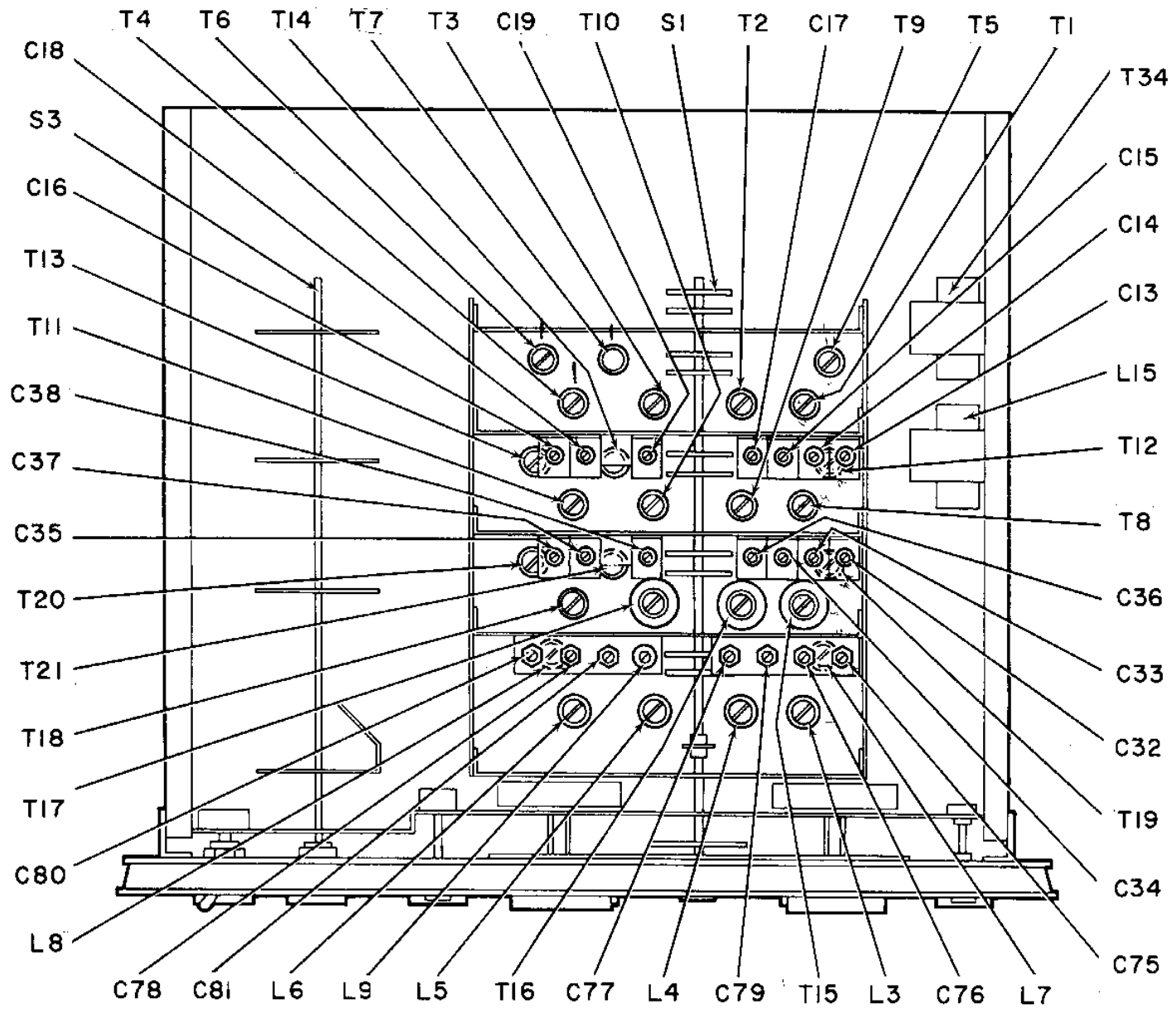
Figure 9. Alignment Adjustments (Bottom Chassis)
