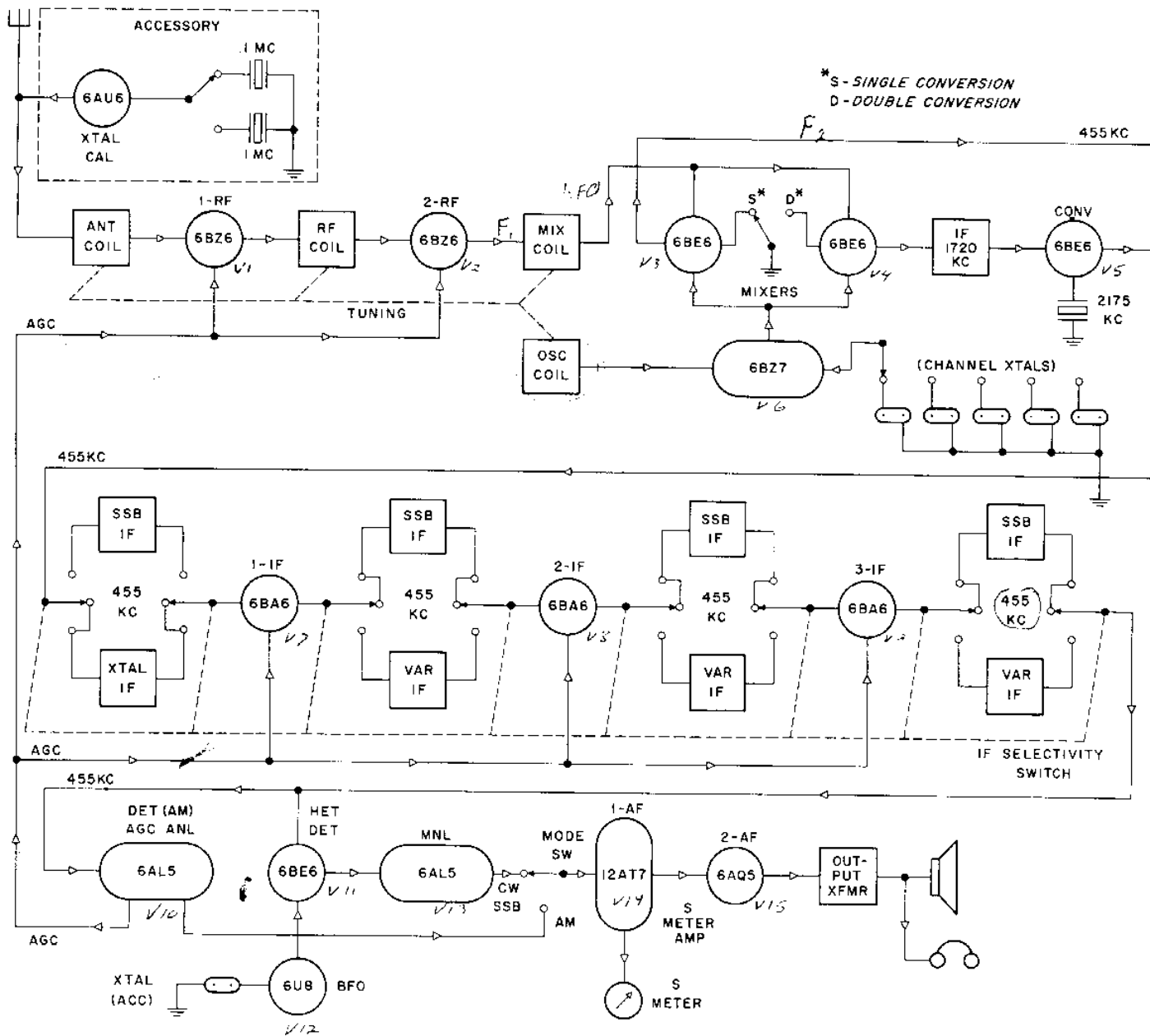
Figure 1. Block Diagram NC-400
