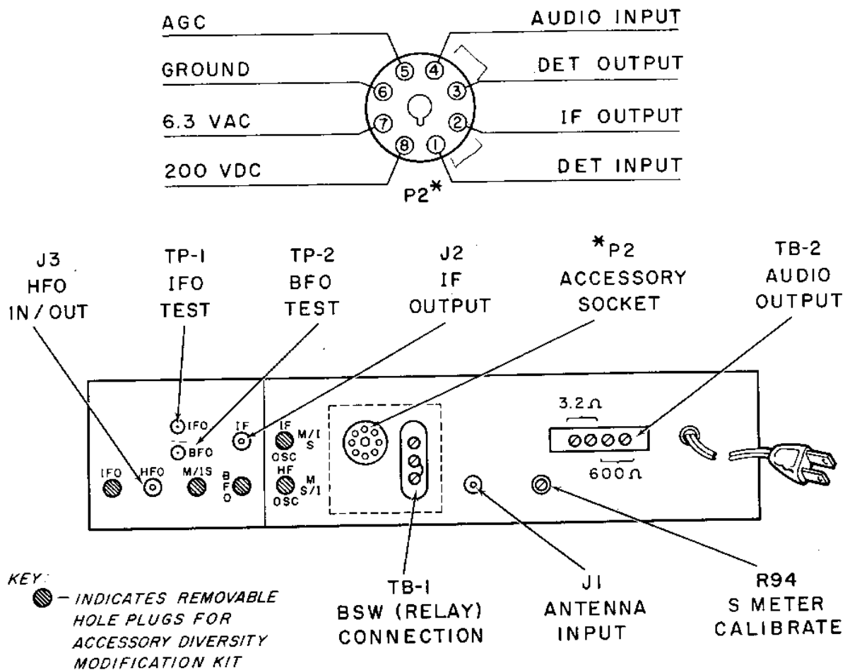
Figure 4. Rear Chassis Panel
