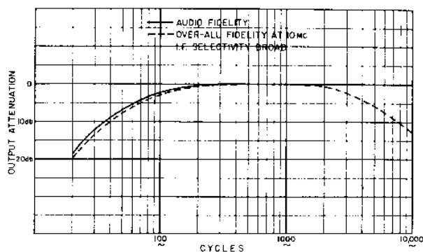
Figure 3. Audio Response
