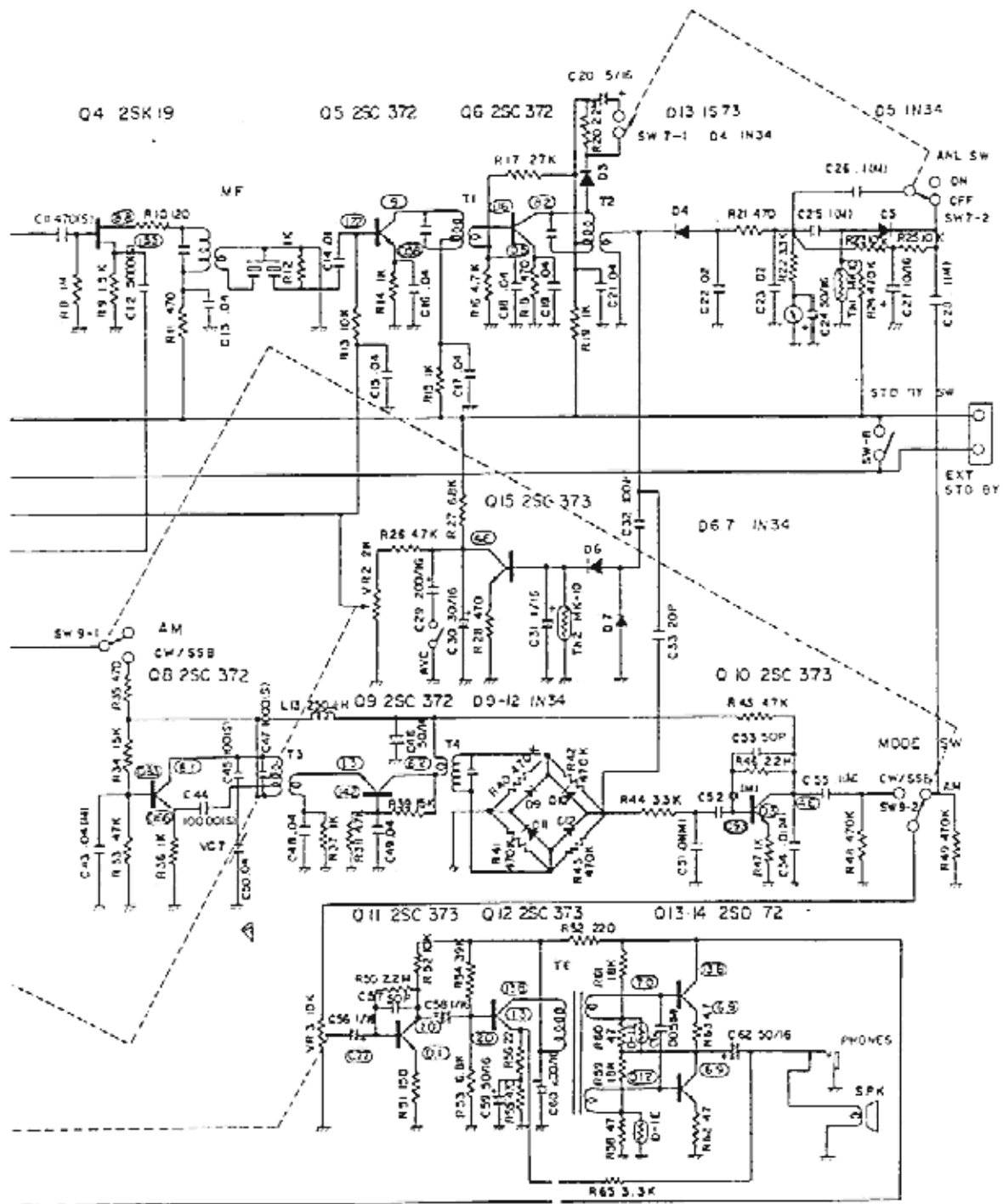
FIG. 4 SCHEMATIC DIAGRAM
