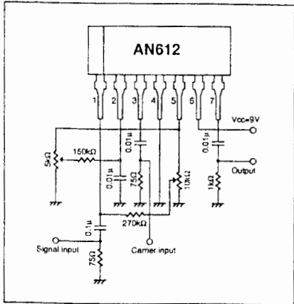
Test Circuit
