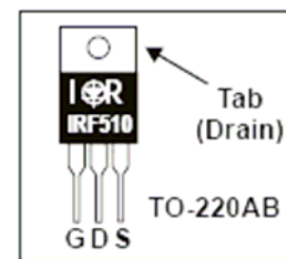
IRF510 FET terminal identification.
