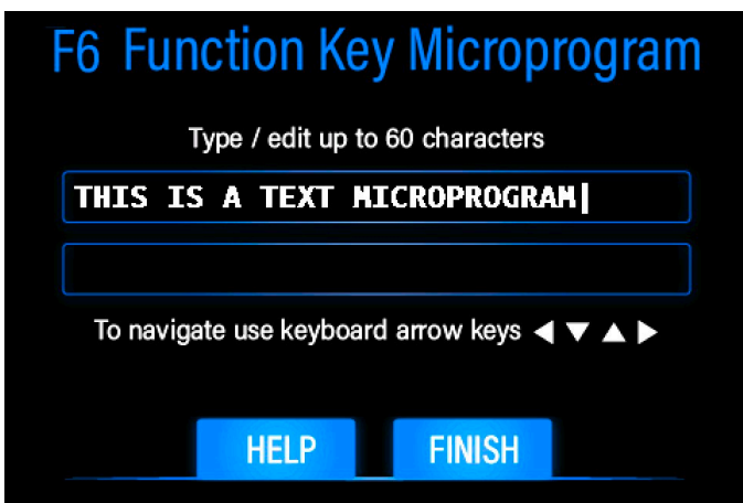
Microprogram Editor
