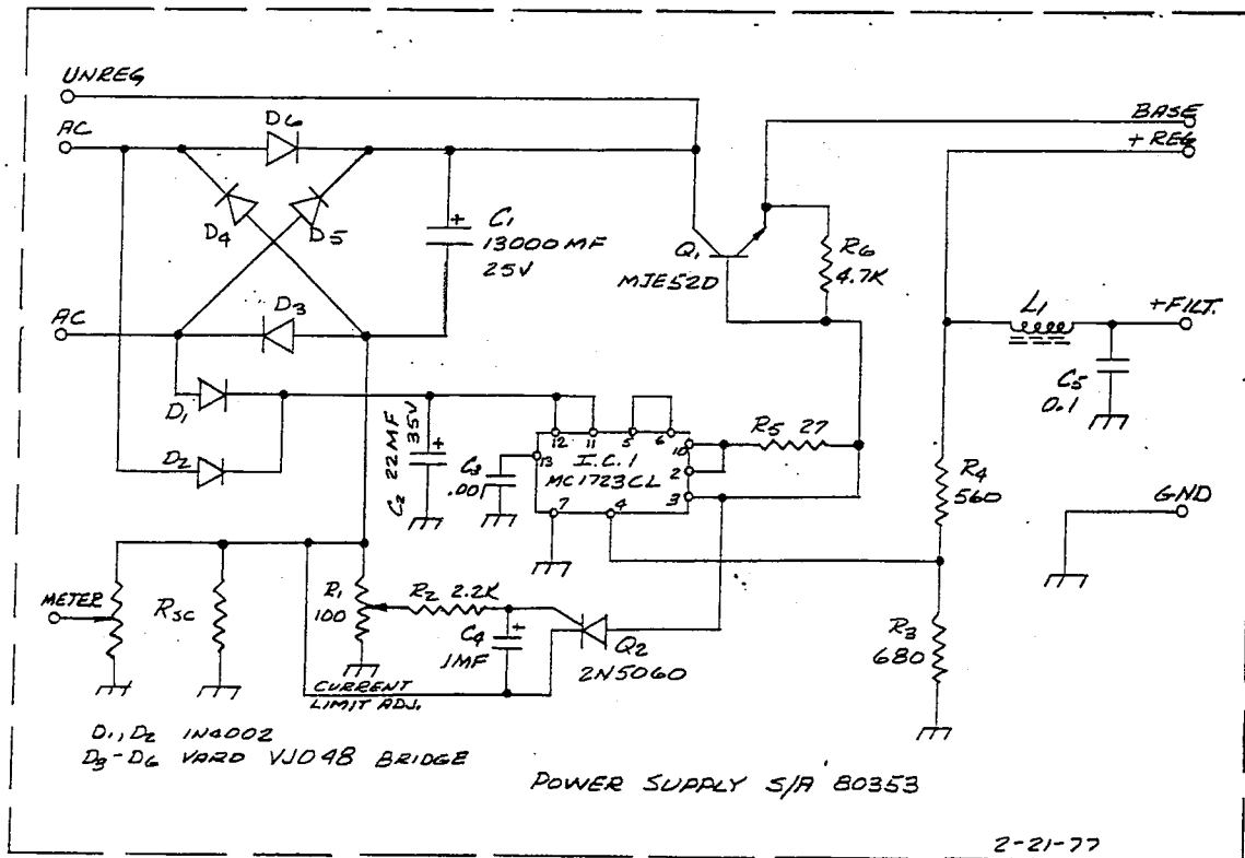
POWER SUPPLY 80353
