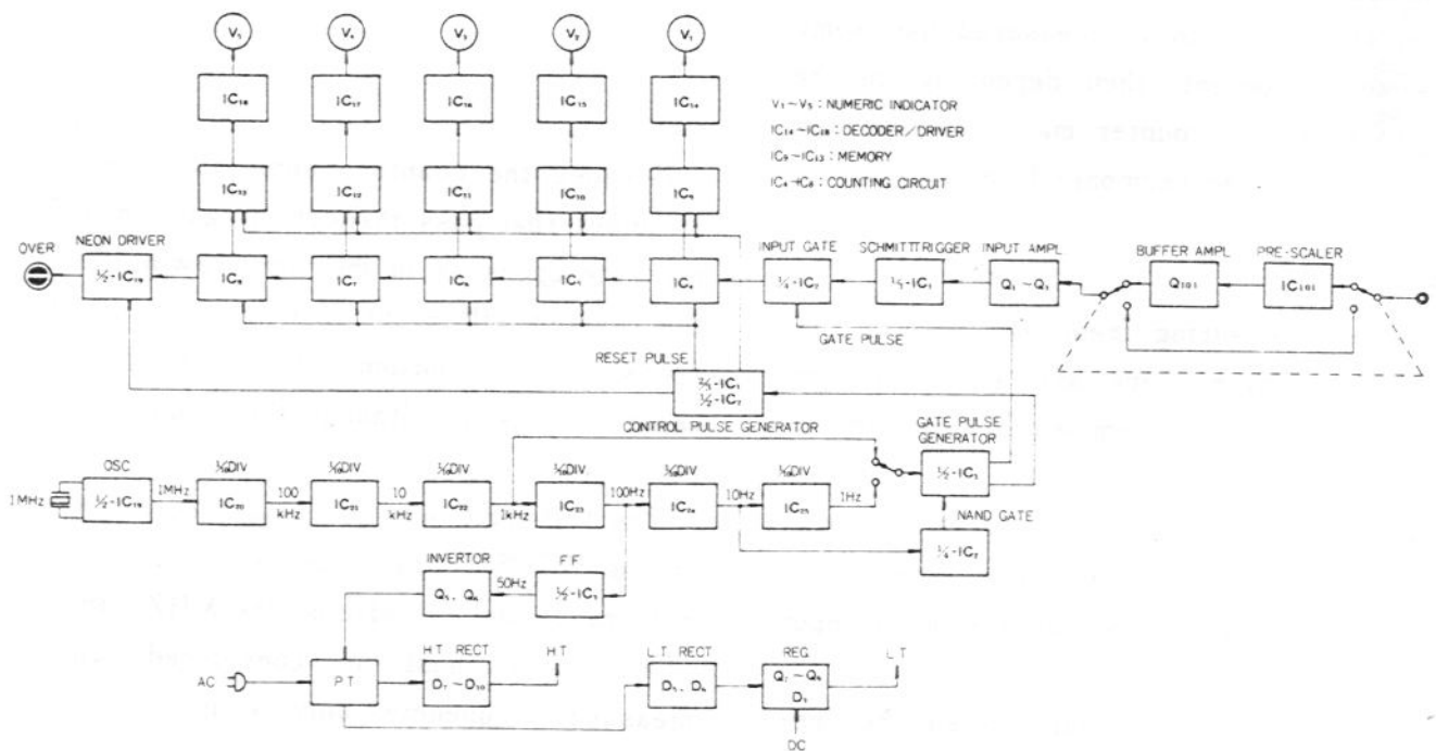
BLOCK DIAGRAM
