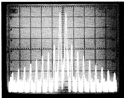
Fig 2—Worst-case spectral display of the FT-1000D transmitter during two-tone intermodulation distortion (IMD) testing. Third-order products are approximately 36 dB below PEP output, and fifth-order products are approximately 42 dB down. Vertical divisions are 10 dB; horizontal divisions are 2 kHz. The transceiver was being operated at 200 W PEP output on 3.9 MHz.
