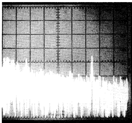
Fig 4—Spectral display of the FT-1000D transmitter output during composite-noise testing. Power output is 200 W at 3.52 MHz (A) and 200 W at 14.02 MHz (B). Vertical divisions are 10 dB; horizontal divisions are 2 kHz. The scale on the spectrum analyzer on which these photos were taken is calibrated so that the log reference level (the top horizontal line on the scale) represents -60 dBc/Hz and the baseline is -140 dBc/Hz. Composite-noise levels between -60 and -140 dBc/Hz may be read directly from the photographs. The carrier, off the left edge of the photographs, is not shown. These photographs show composite transmitted noise at frequencies 2 to 20 kHz offset from the carrier. The FT-1000's composite transmitted noise is composed mostly of broadband amplifier noise, not phase noise.
