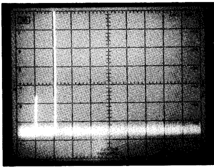
Fig 1—Yaesu FT-1000D worst-case spectral display. Horizontal divisions are 10 MHz; vertical divisions are 10 dB. Output power is approximately 194 W at 21.1 MHz. All harmonics and spurious emissions are at least 45 dB below peak fundamental output. The FT-1000D complies with current FCC specifications for spectral purity for equipment in this power-output class and frequency range.
