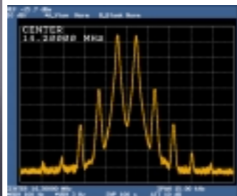
Typical TX IMD: Class A (25W Output)
