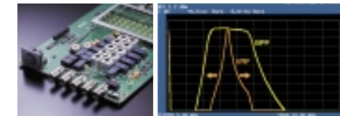
VRF Features Large, High-Q Coils and High-Quality Relays VRF Typical Bandpass Response (3.5 MHz)
