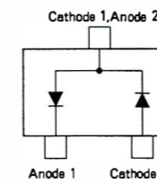
1SS302 (C3) (D1003, 1010)
