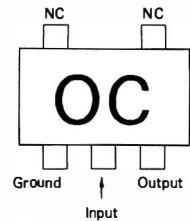
RN5RL30AA-TR (OC) (Q5001)
