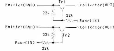
IMH5 CIRCUIT DIAGRAM
