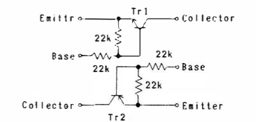
IMD2 CIRCUIT DIAGRAM
