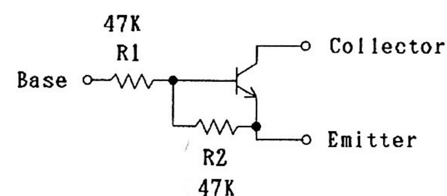
DTC144EK CIRCUIT DIAGRAM
