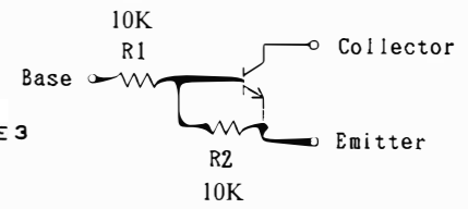
DTC114EK CIRCUIT DIAGRAM
