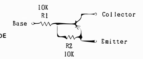
DTA114EK CIRCUIT DIAGRAM
