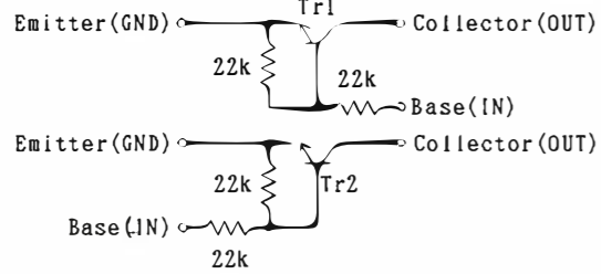
IMH5 CIRCUIT DIAGRAM
