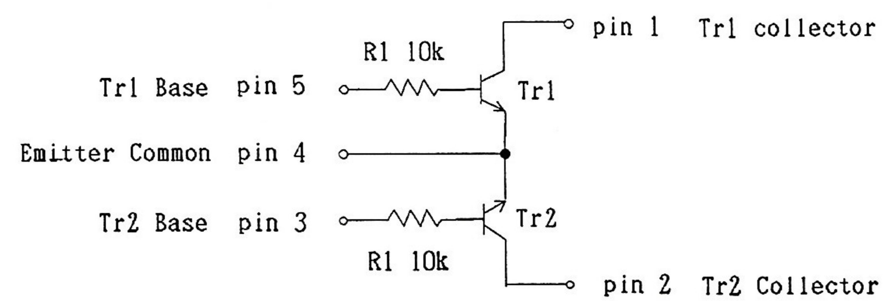
FMG4 CIRCUIT DIAGRAM
