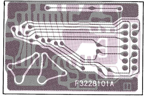
solder side
