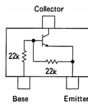
DTC124EK (25) (Q302)
