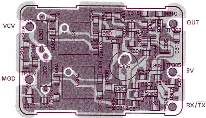
component side
