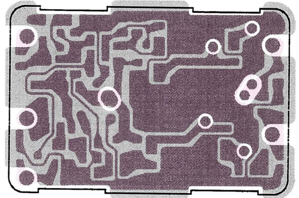
chip-only side
