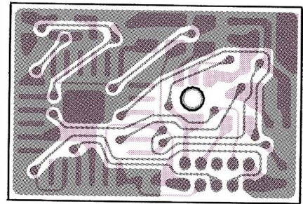
solder side
