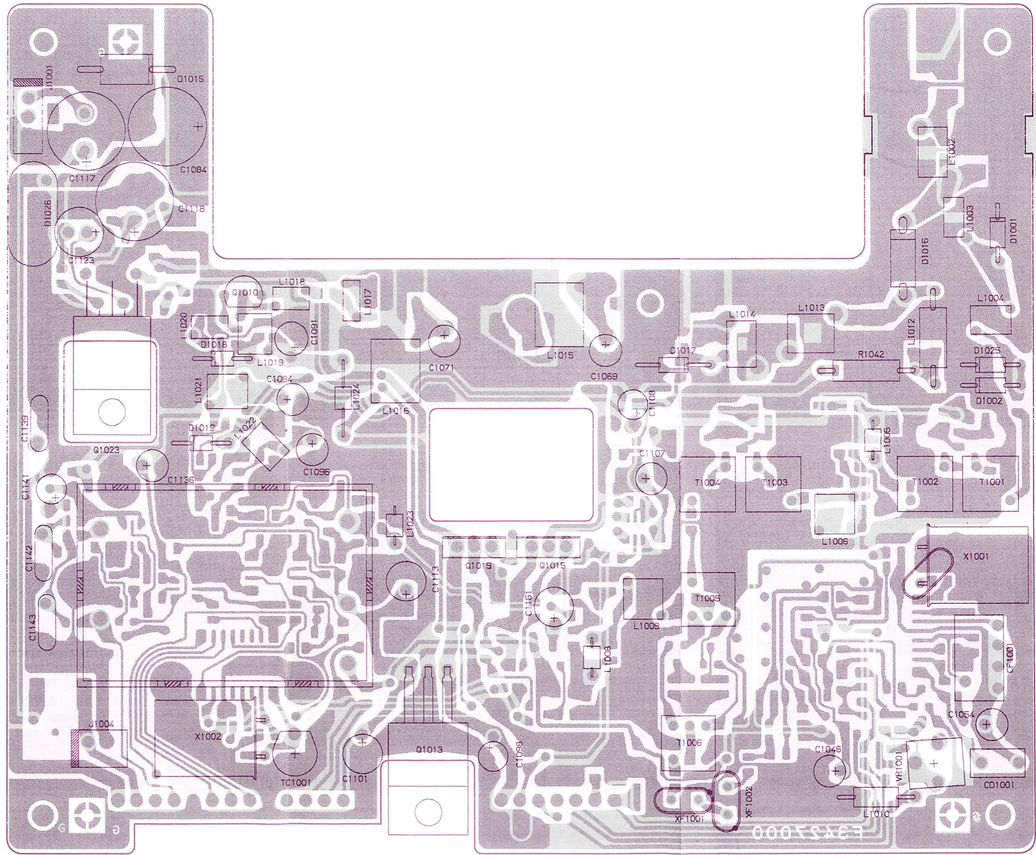
component side
