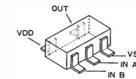
TC4S71F (C4) (Q2001)
