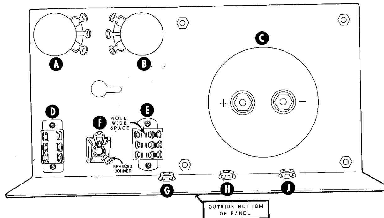
PICTORIAL 6
