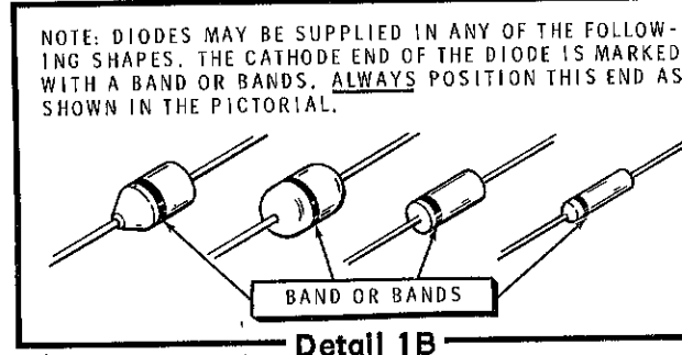
Detail 1B
