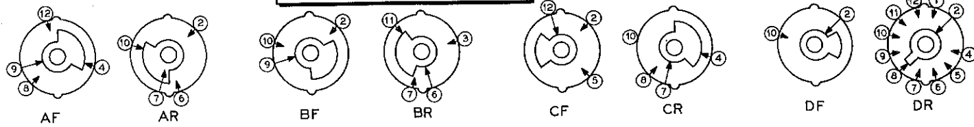
ROTARY SWITCH WAFERS
