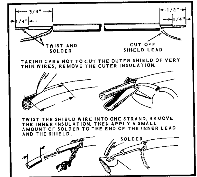
Detail 7C
