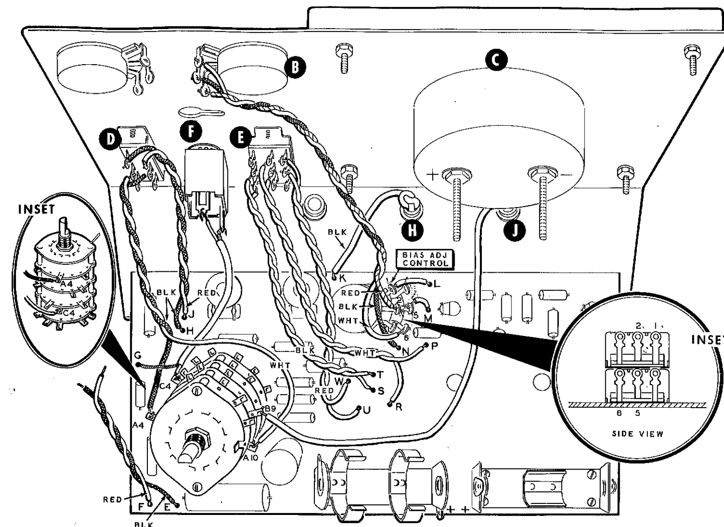
PICTORIAL 8
