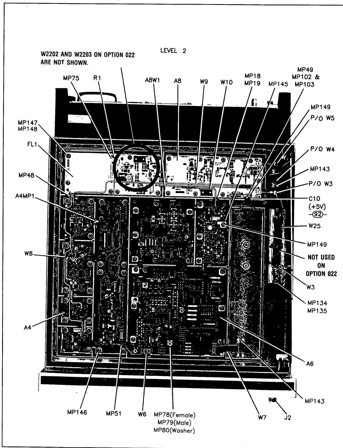
Figure 6-7. Top Internal View Level 2
