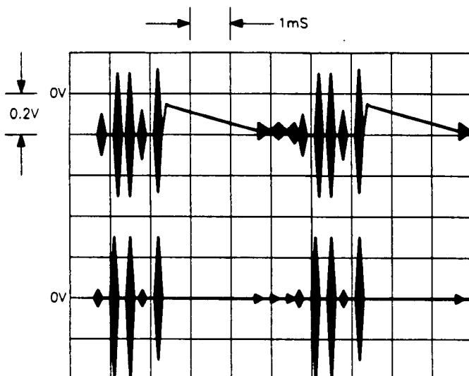
Figure 4. Beatnote Amplifier.
