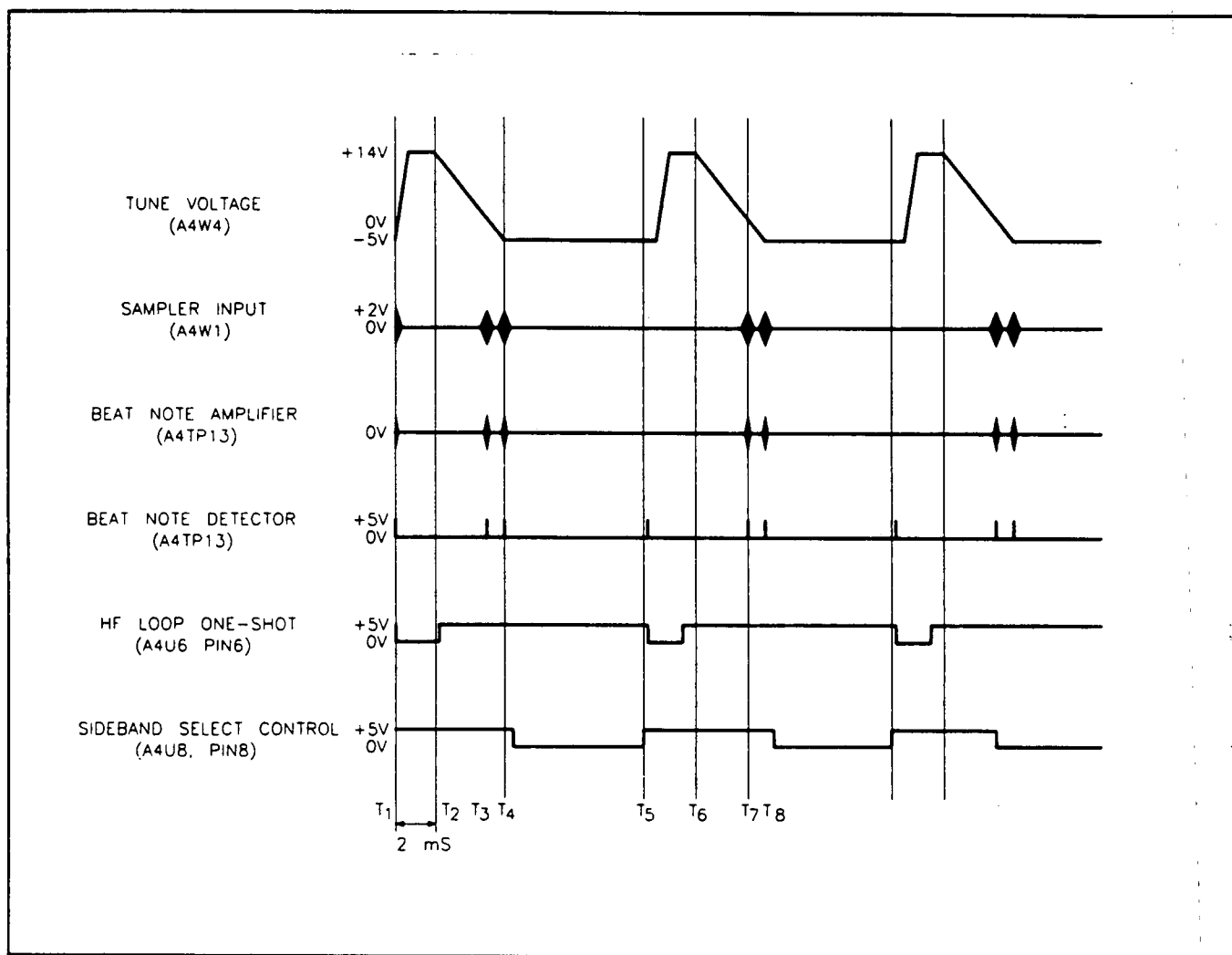
Figure 1. High Frequency Loop Control Timing Diagram.
