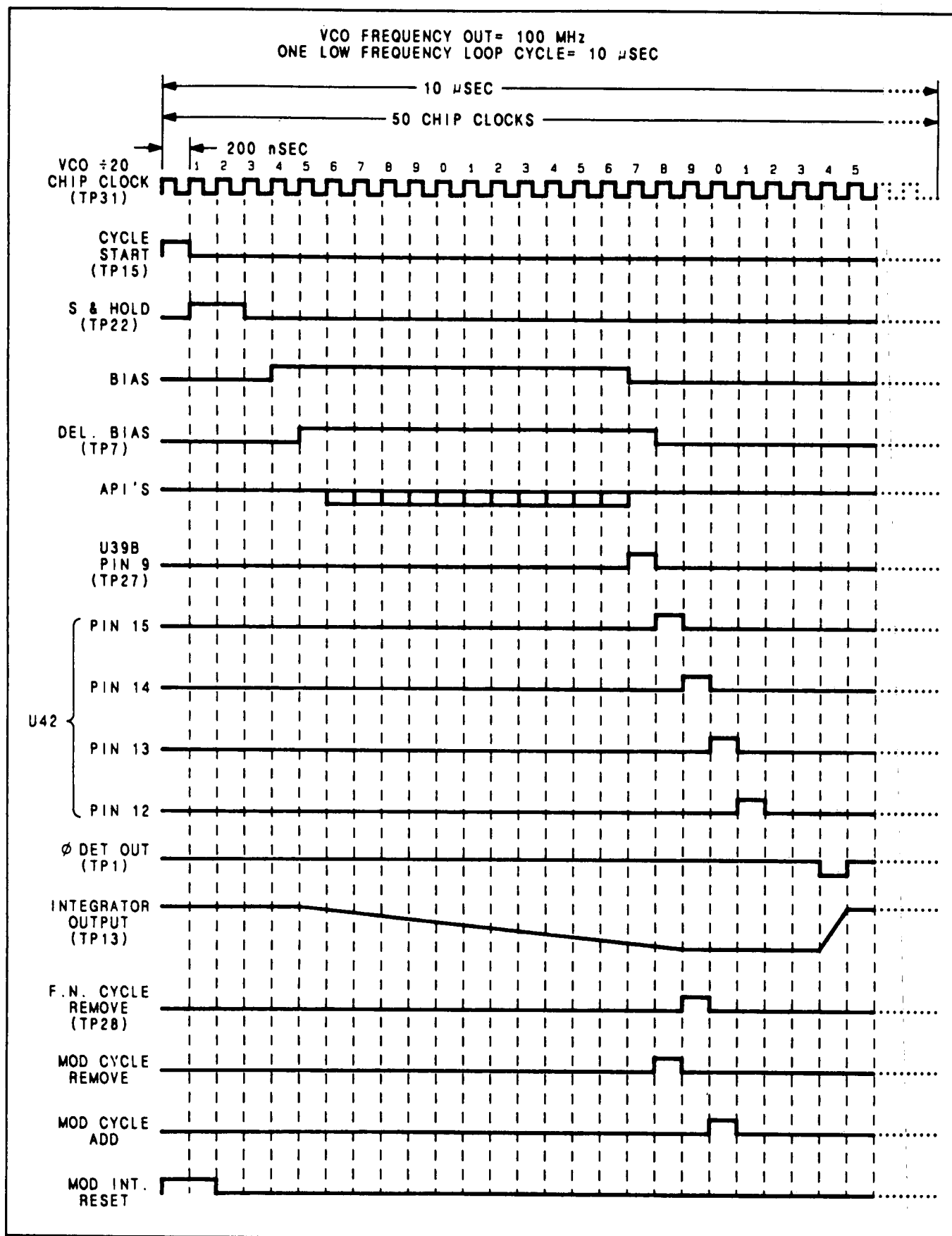
Figure 8. Low Frequency Loop Timing Diagram.
