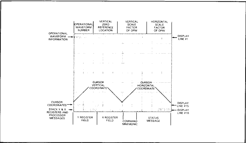
Figure 5-4. Typical character display of STORED mode.
