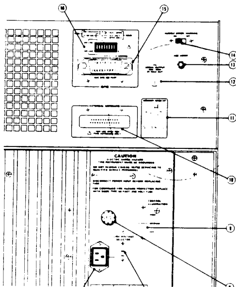
Figure C. Locator for 7854 rear-panel controls, connectors, and indicators.
