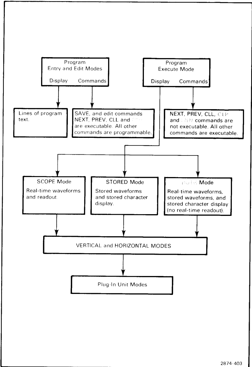
Figure 9-1. The 7854 hierarchy of operational modes.
