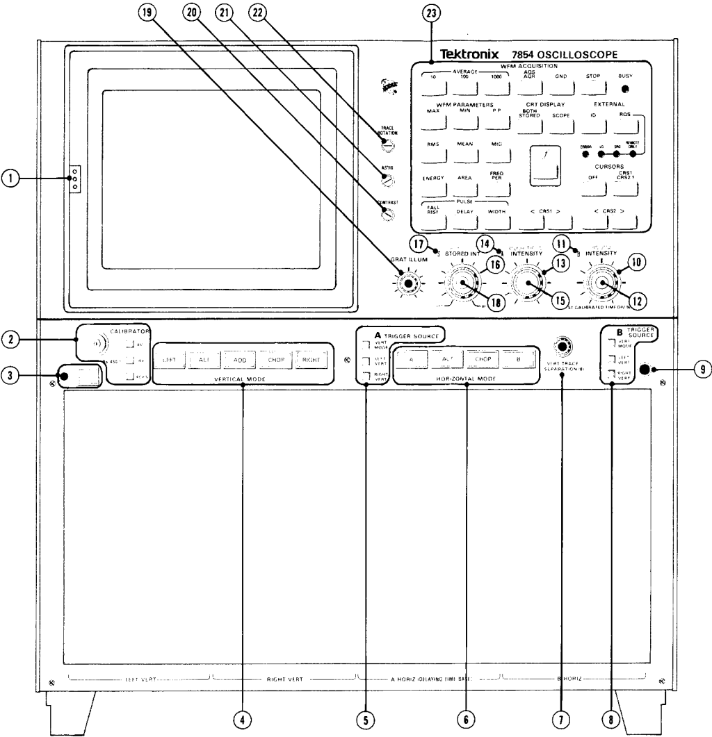
Figure A. Locator for 7854 front-panel controls, connectors, and indicators.
