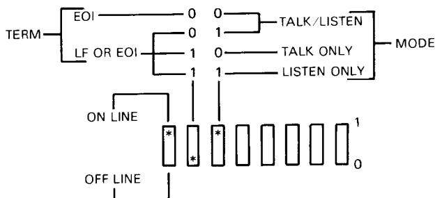
Figure 7-2. Address and mode selection.
