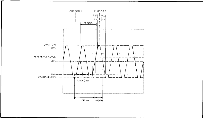
Figure 5-5. Time-parameter relationships.
