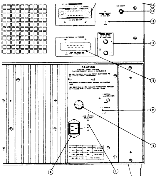
Figure C. Locator for 7854 rear-panel controls, connectors, and indicators.
