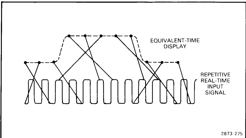
Figure 5-2. The input pulse of a repetitive signal is reconstructed using equivalent-time random sampling.
