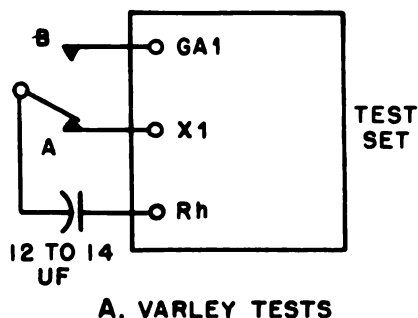
Figure 17. Connections for use of capacitor and switch to compensate for foreign voltage during test.
