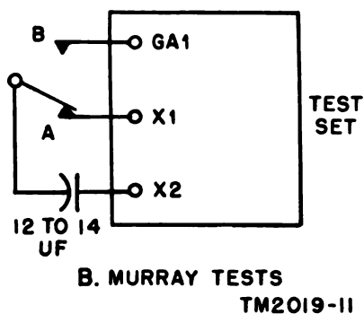
Figure 17. Connections for use of capacitor and switch to compensate for foreign voltage during test.
