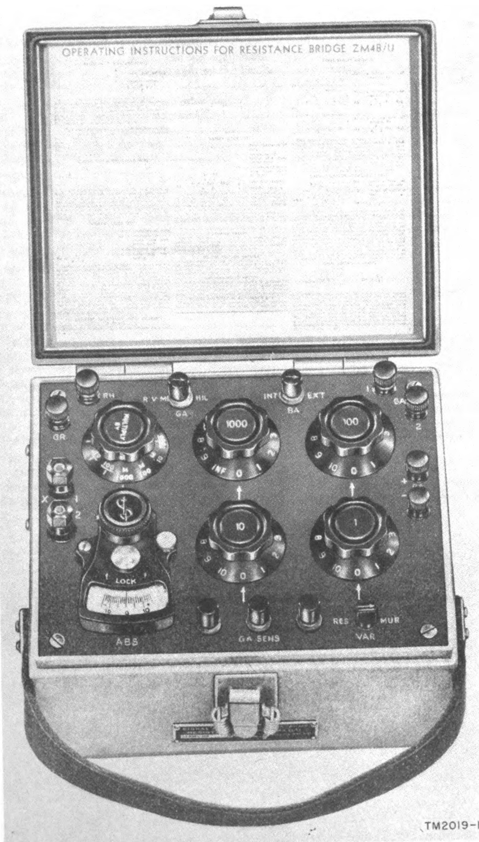
Figure 1. Resistance Bridge ZM-4B/U.
