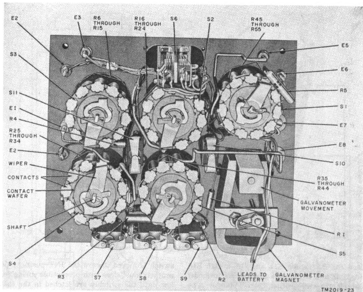
Figure 22. Resistance Bridge ZM-4A/U, bottom view.
