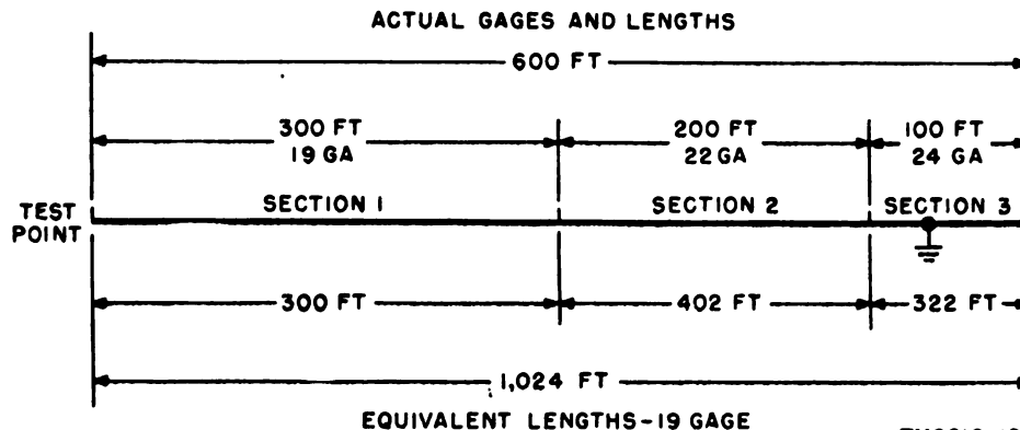
Figure 12. Grounded conductor in nonuniform gauge circuit.
