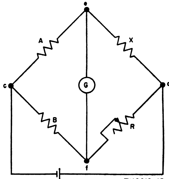
Figure 15. Basic bridge circuit.
