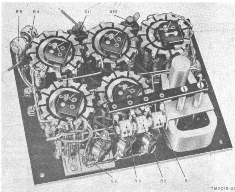
Figure 23. Resistance Bridge ZM-4B/U, bottom view.
