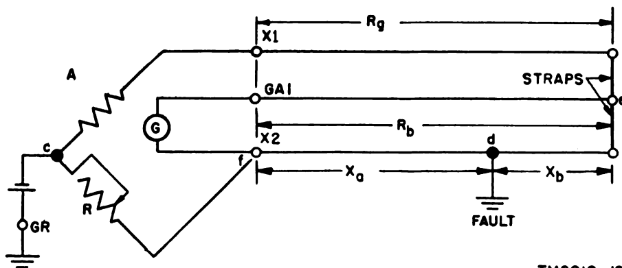
Figure 19. Hilborn loop test circuit, schematic diagram.
