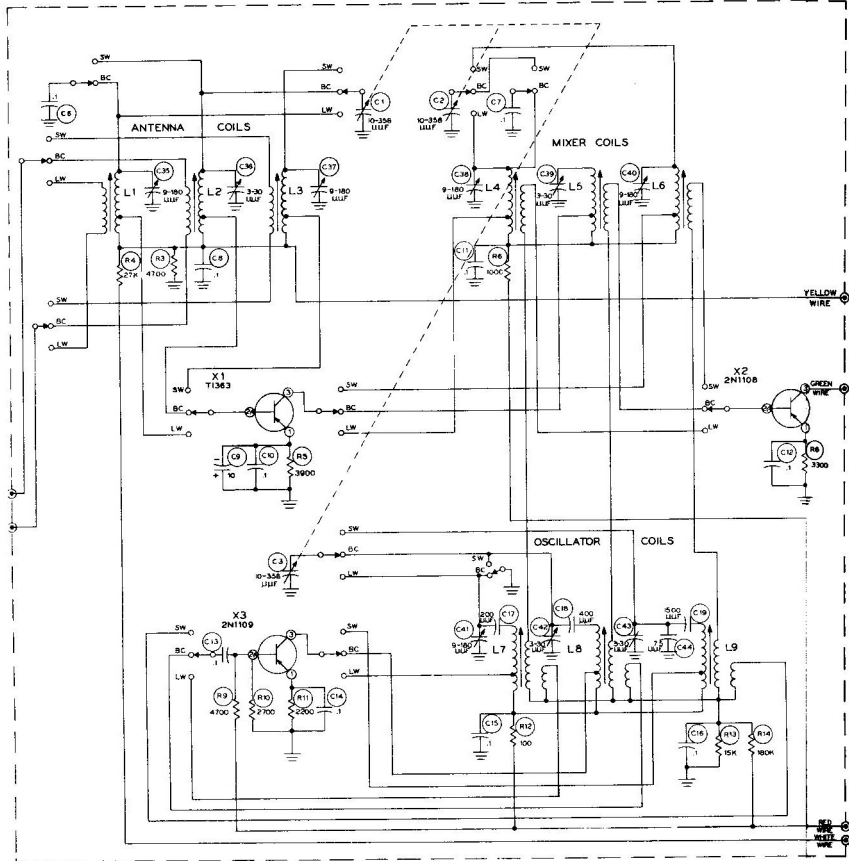
PREASSEMBLED PREALIGNED TUNING UNIT
