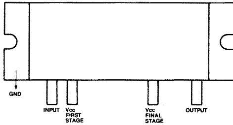
SC-1022 IC1 (45W VHF RF POWER AMP)
