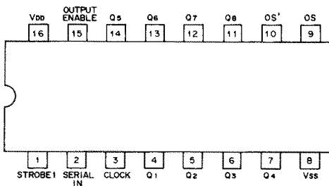
μPD4094BC (IC-228A: U.S.A., Asia) IC5 (8-STAGE SHIFT REGISTER)
