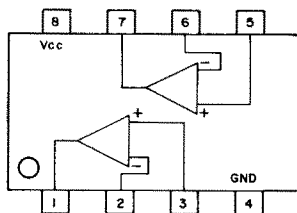
NJM4558D IC7 (DUAL NOISE LOW AMP)
