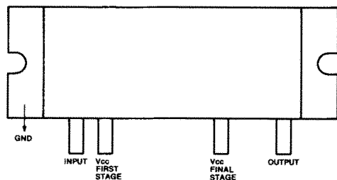
SC-1019 IC1 (25W VHF RF POWER AMP)
